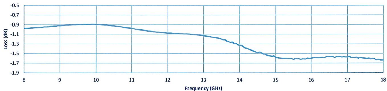
Insertion Loss
