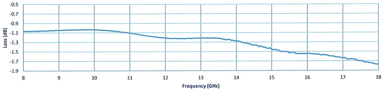
Insertion Loss
