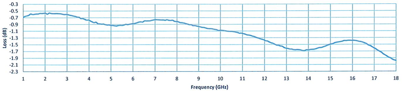
Insertion Loss
