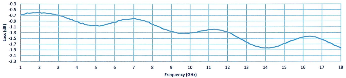
Insertion Loss
