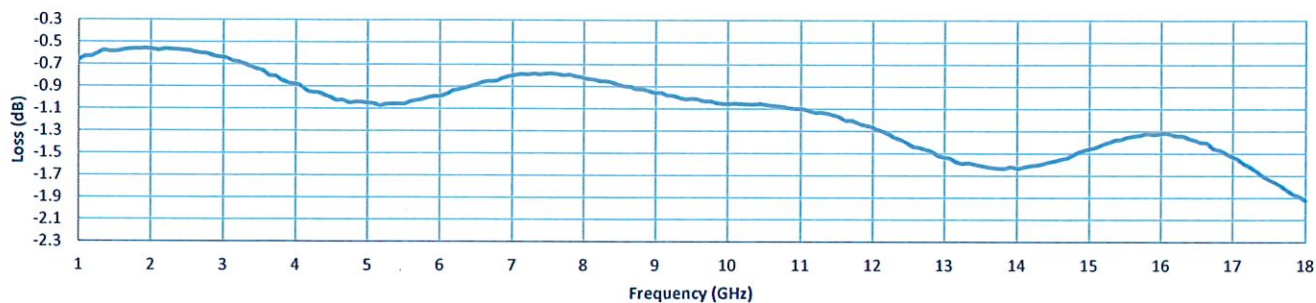
Insertion Loss
