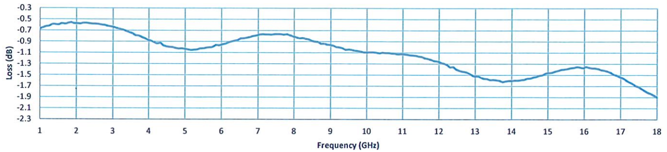
Insertion Loss
