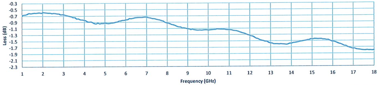
Insertion Loss
