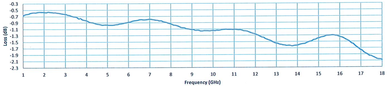
Insertion Loss
