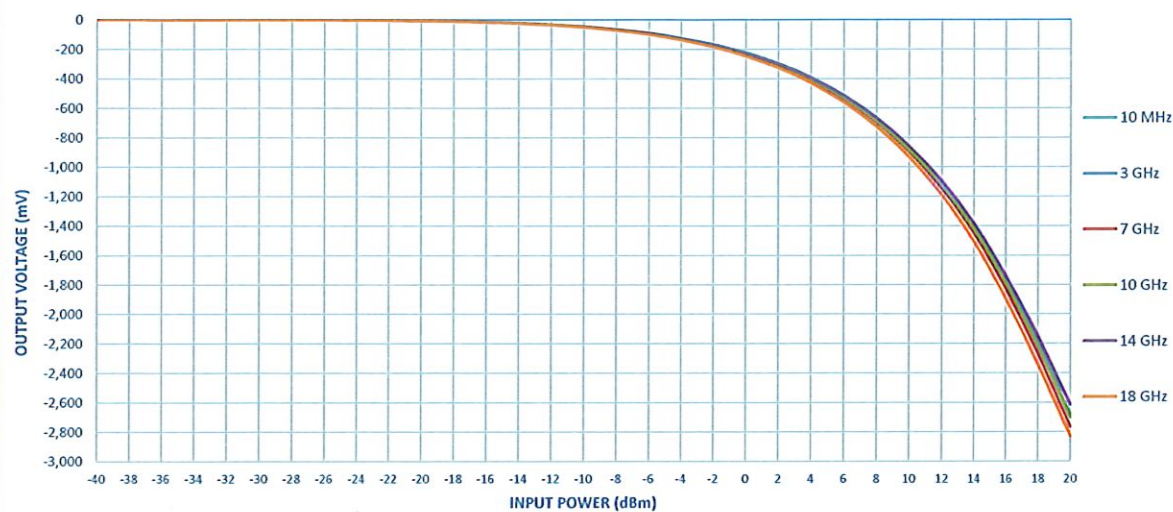
Transfer Curve
