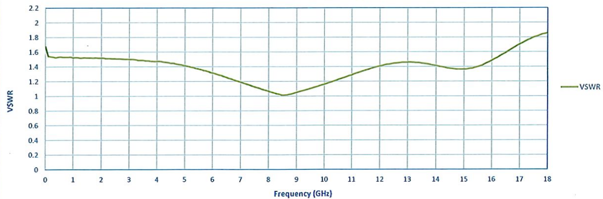
VSWR Vs Frequency
