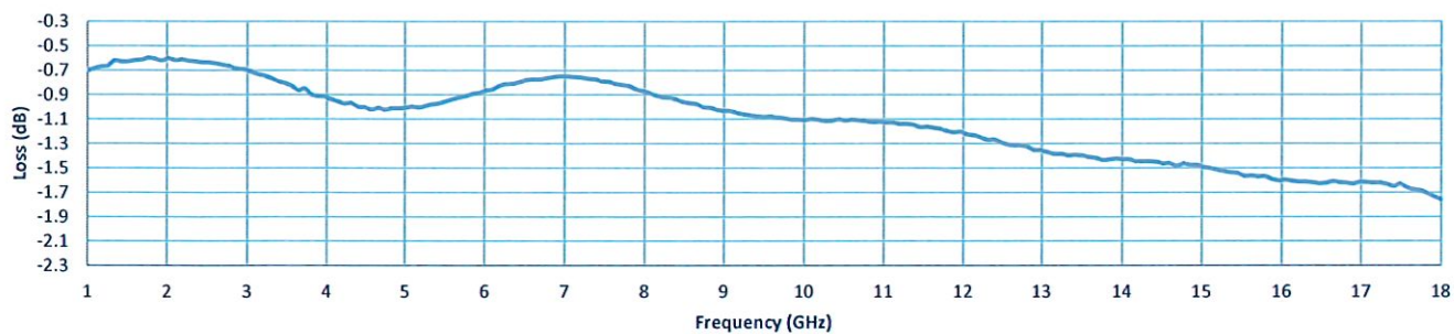
Insertion Loss
