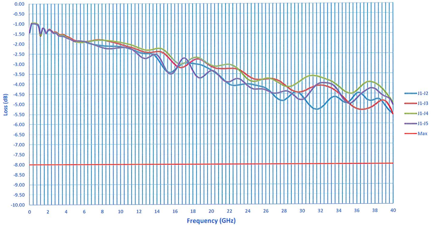
Insertion Loss
