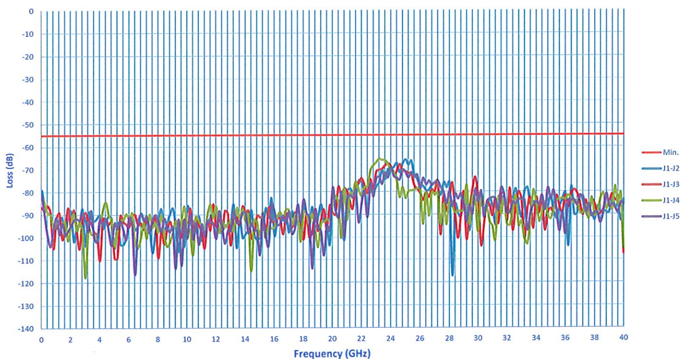
Isolation
