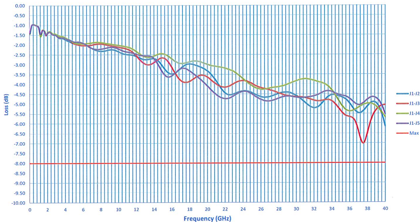
Insertion Loss
