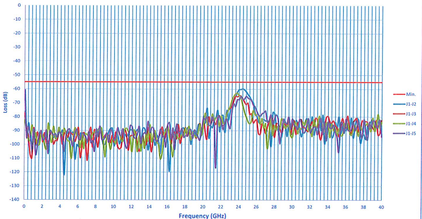
Isolation
