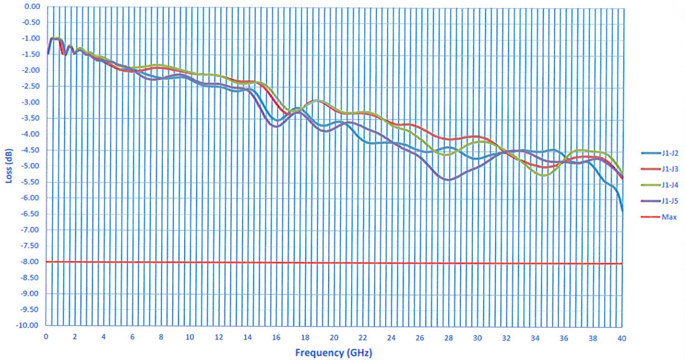
Insertion Loss
