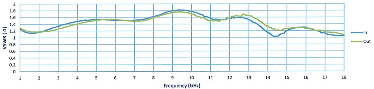
VSWR @ -20dBm
