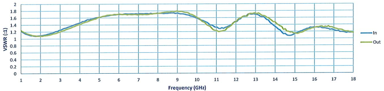
VSWR @ -20dBm
