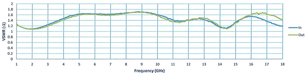
VSWR @ -20dBm
