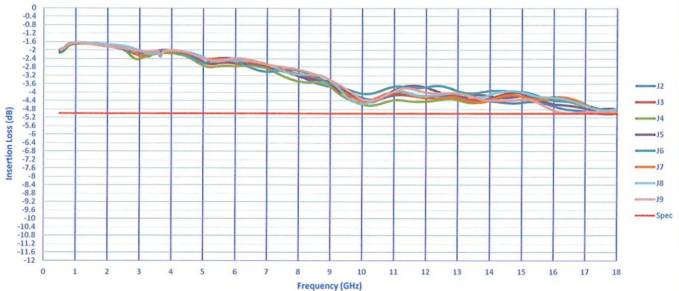
Insertion Loss
