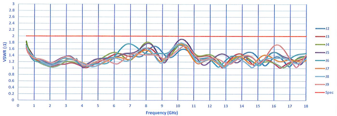
Input VSWR (On)
