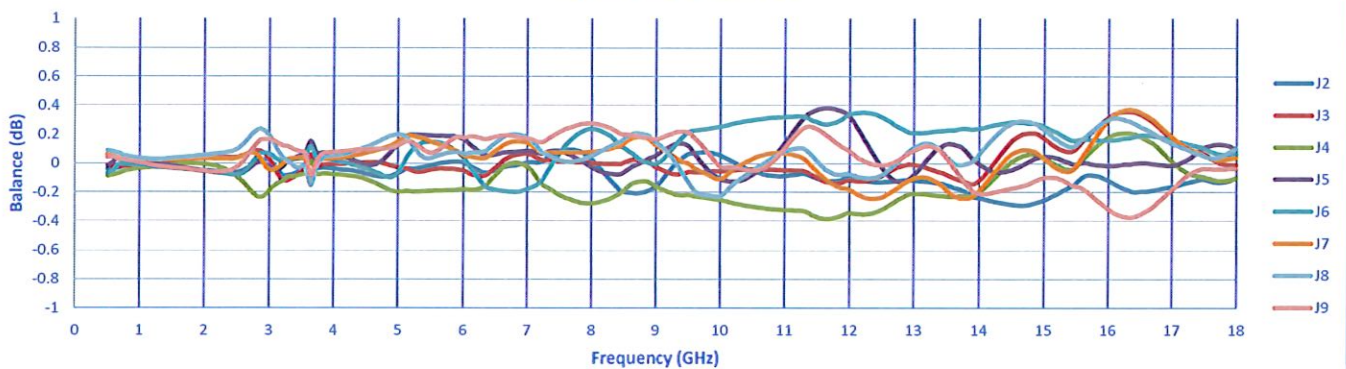
Amplitude Balance
