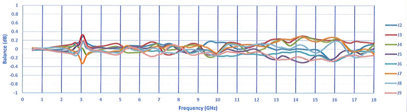
Amplitude Balance
