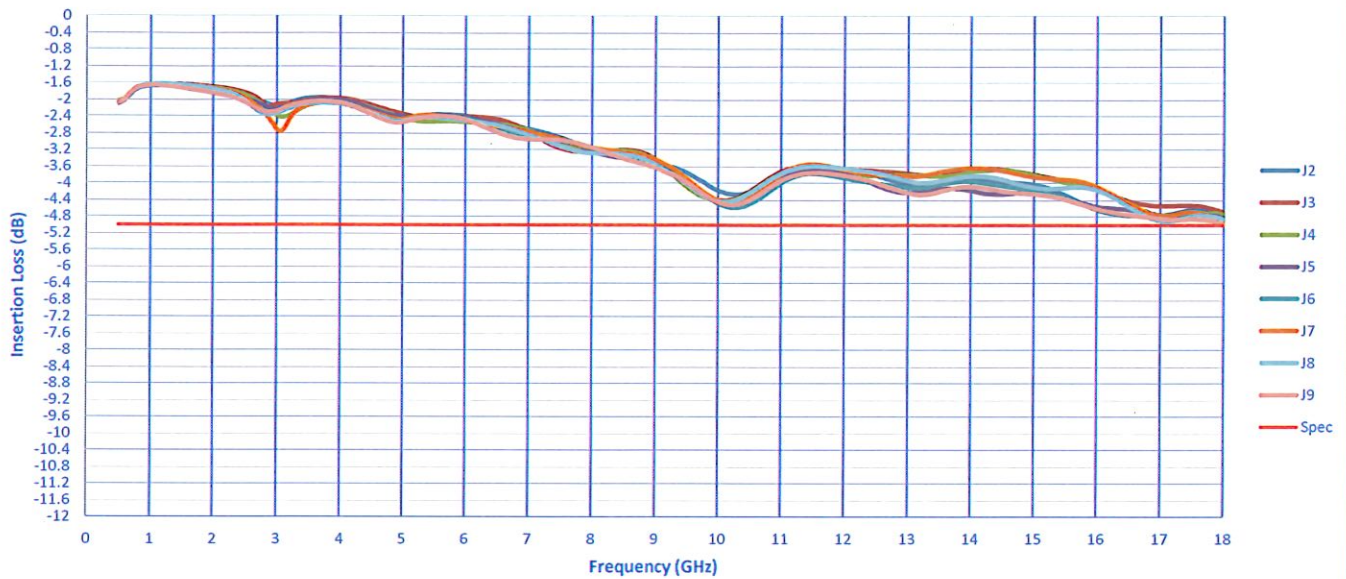
Insertion Loss
