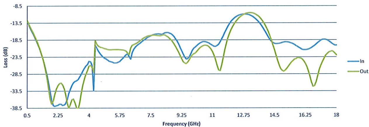
Return Loss
