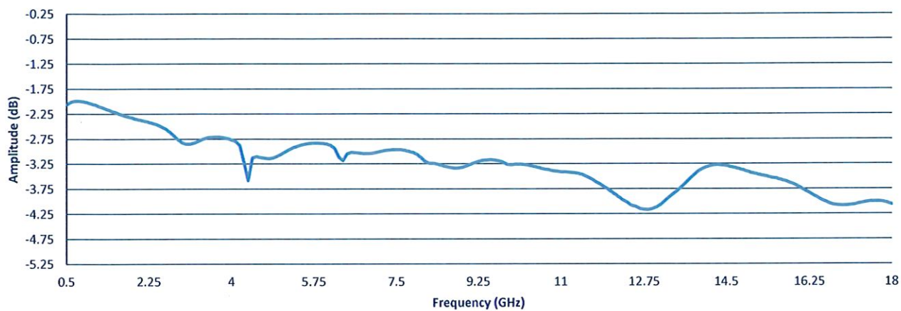
Insertion Loss
