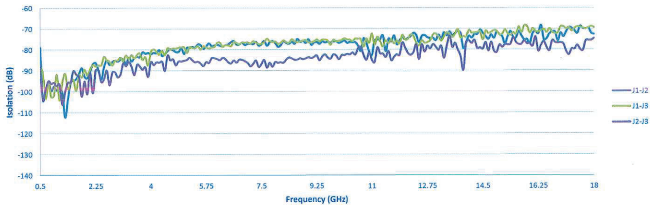
Isolation
