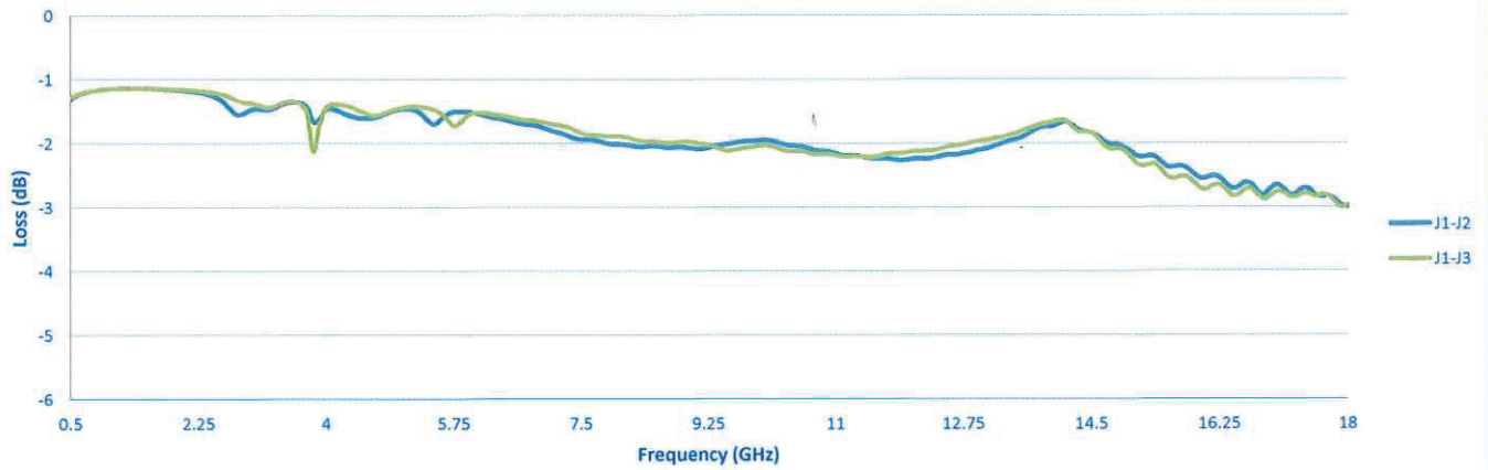
Insertion Loss
