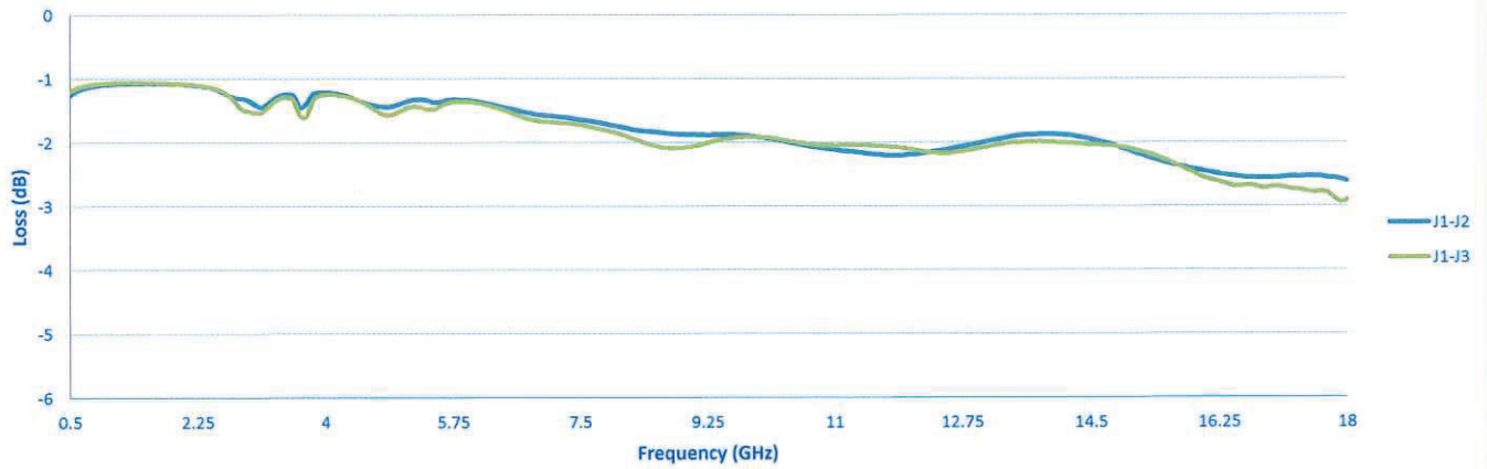
Insertion Loss
