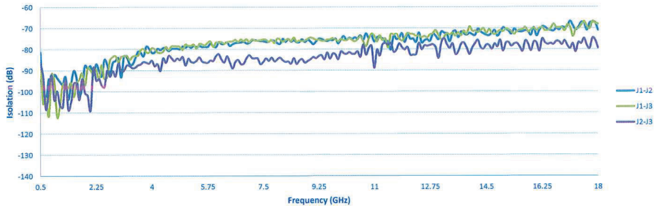
Isolation
