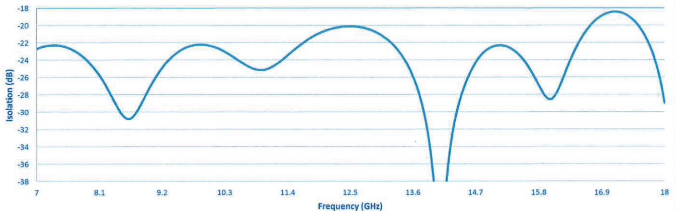
Isolation
