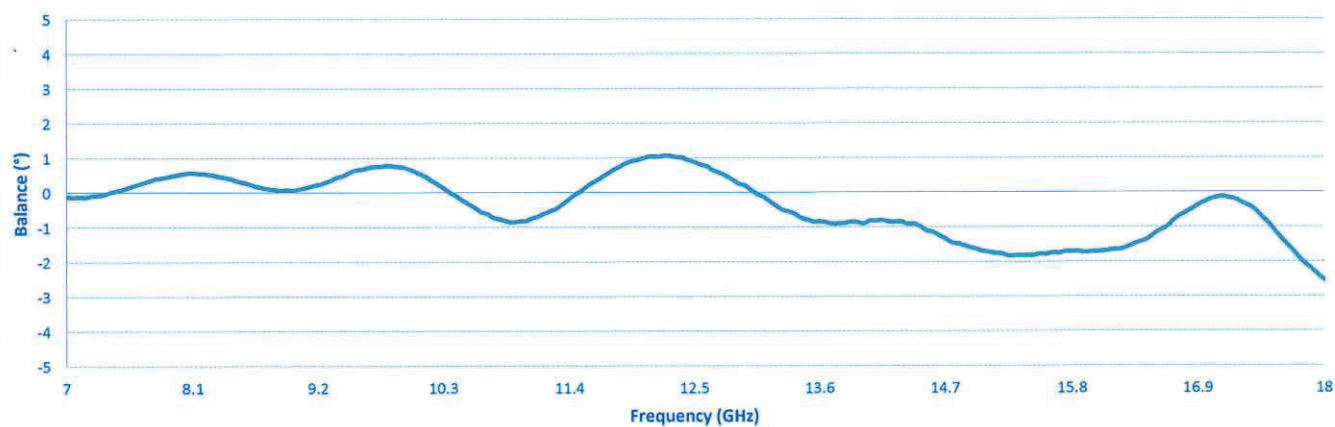
Phase Balance
