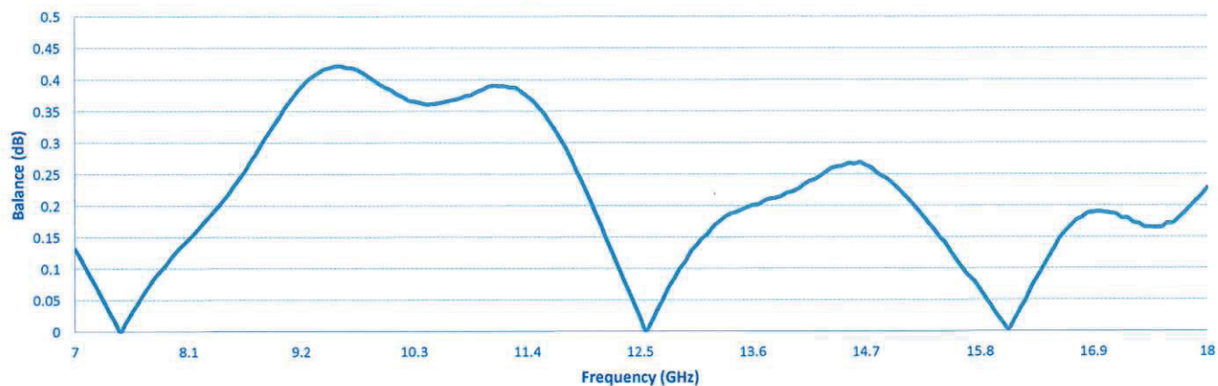
Amplitude Balance
