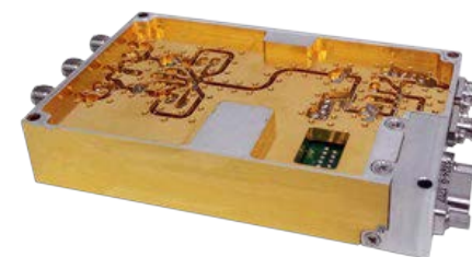
0.5 to 18 GHz, Custom Phase ( \pm 10^\circ ) & Amplitude ( \pm 1.5 dB) Matched Integrated Modules/Assemblies
