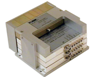
0.02 to 3 GHz, SP8T Switch Matrix Assembly
