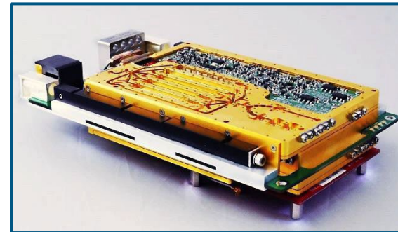
0.1 to 18 GHz Transceiver (Phase III)
