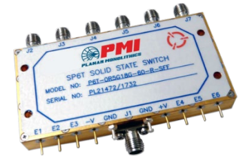
0.5 to 18 GHz SP6T Reflective Switch
