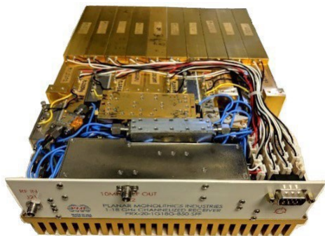
1 to 18 GHz Channelized Receiver
