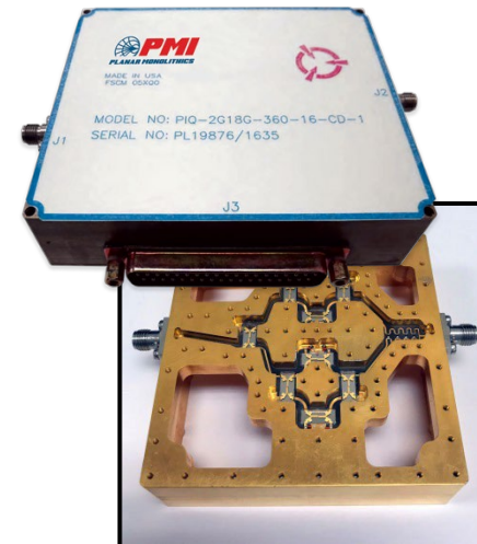
2 to 18 GHz, High Performance I/Q Vector Modulator
