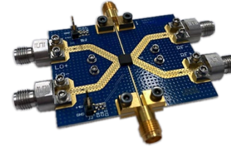
Evaluation Board for PIQ-1-SMT Integrated Broadband IQ Vector Modulator
