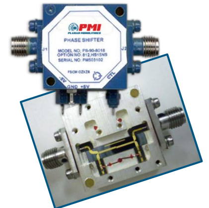
1.1 to 1.12 GHz, 180° Bi-Phase Modulator/Phase Shifter
