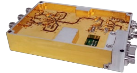
0.5 to 18 GHz, Custom Phase ( \pm 10^\circ ) & Amplitude ( \pm 1.5 dB) Matched Integrated Modules/ Assemblies
