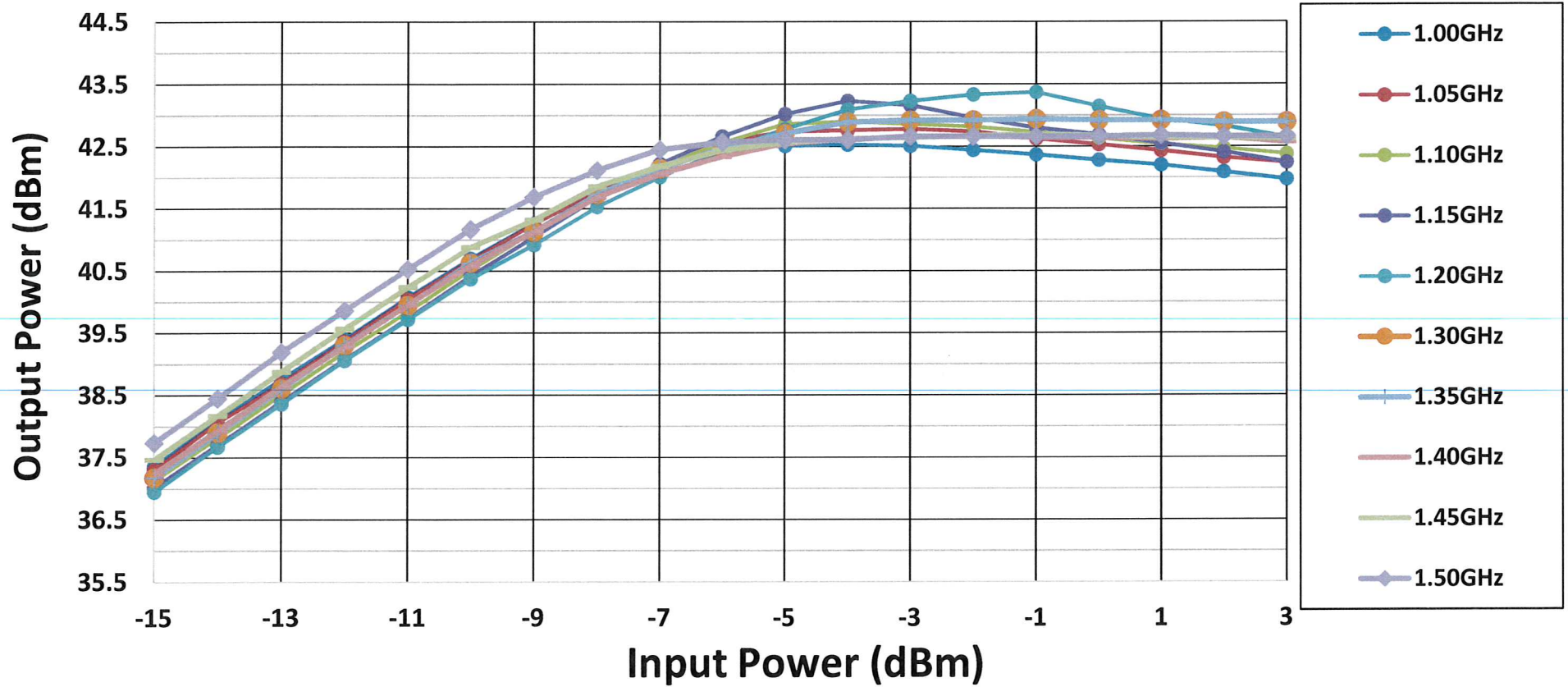
Output Power Vs Input Power
