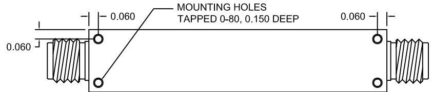
VIEW FORM BOTTOM
