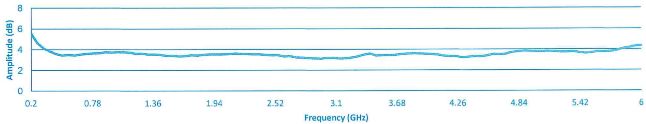
Noise Figure
