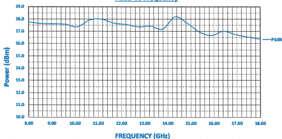
P1dB Vs Frequency
