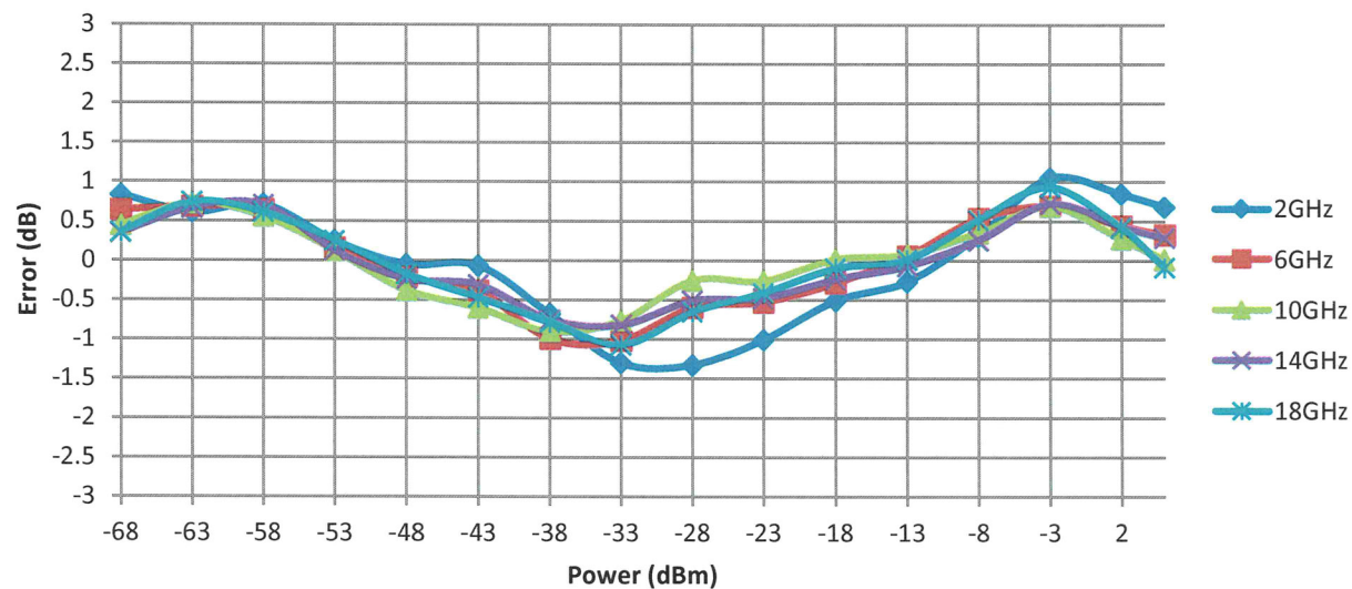
Linearity Error
