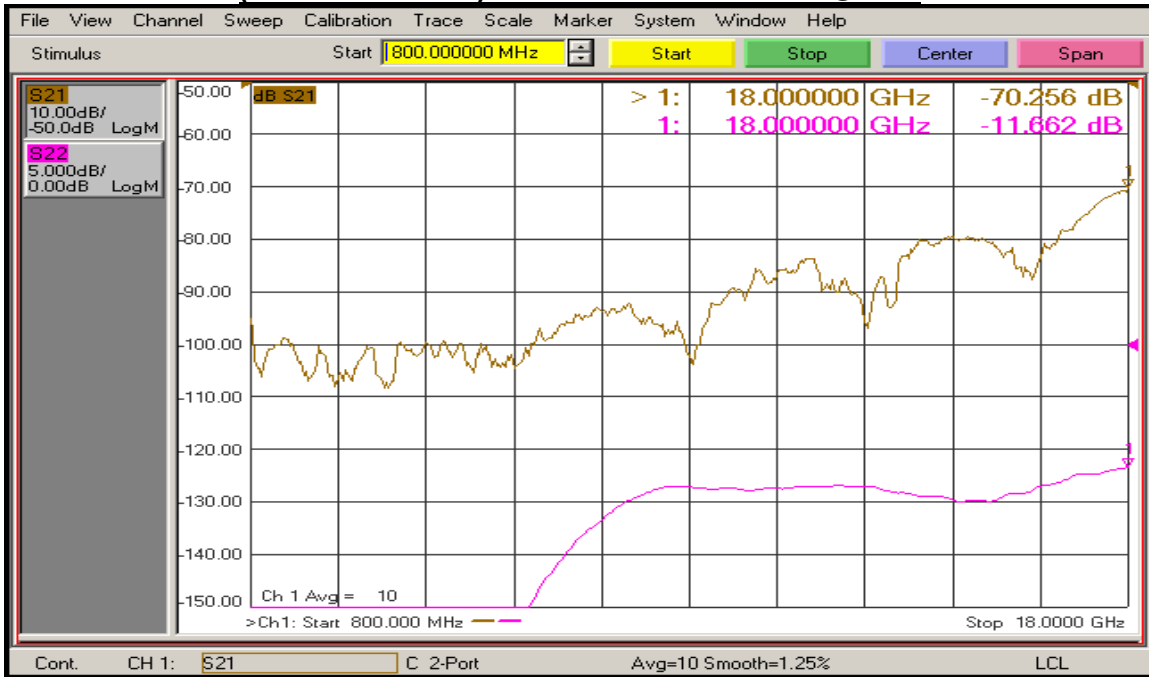
(J8 - J1 with J6 ON) Isolation and Return Loss @ 25°C
