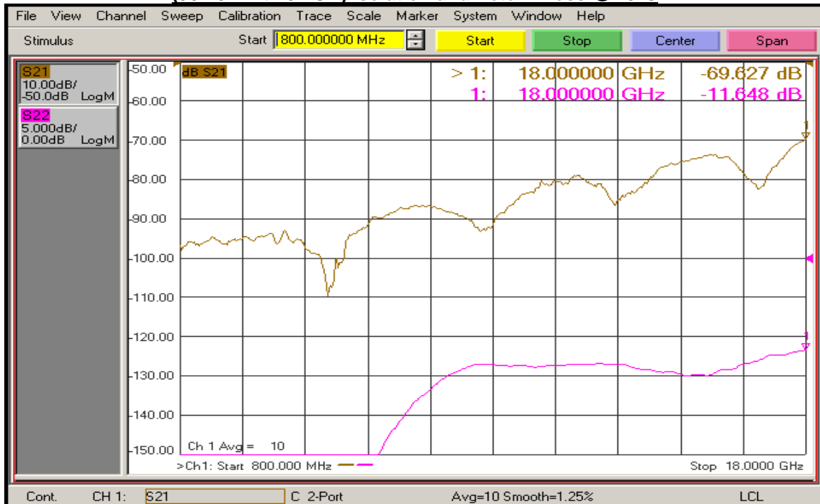
(J8 - J1 with J2 ON) Isolation and Return Loss @ 25°C
