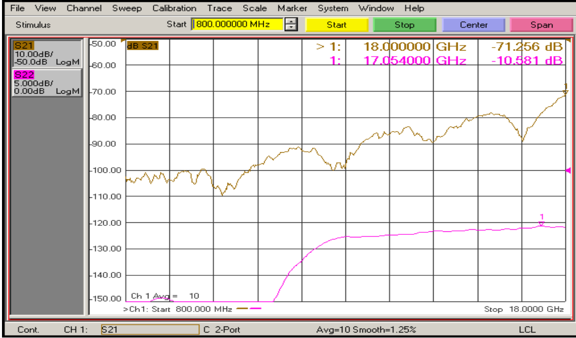
(J8 – J2 with J4 ON) Isolation and Return Loss @ 25°C
