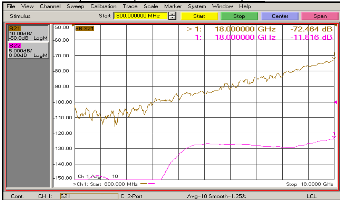
(J8 – J4 All Off) Isolation and Return Loss @ 25°C
