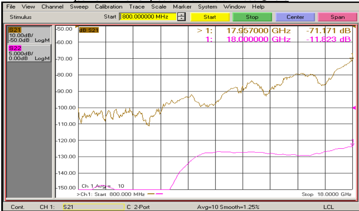
(J8 – J4 with J2 ON) Isolation and Return Loss @ 25°C
