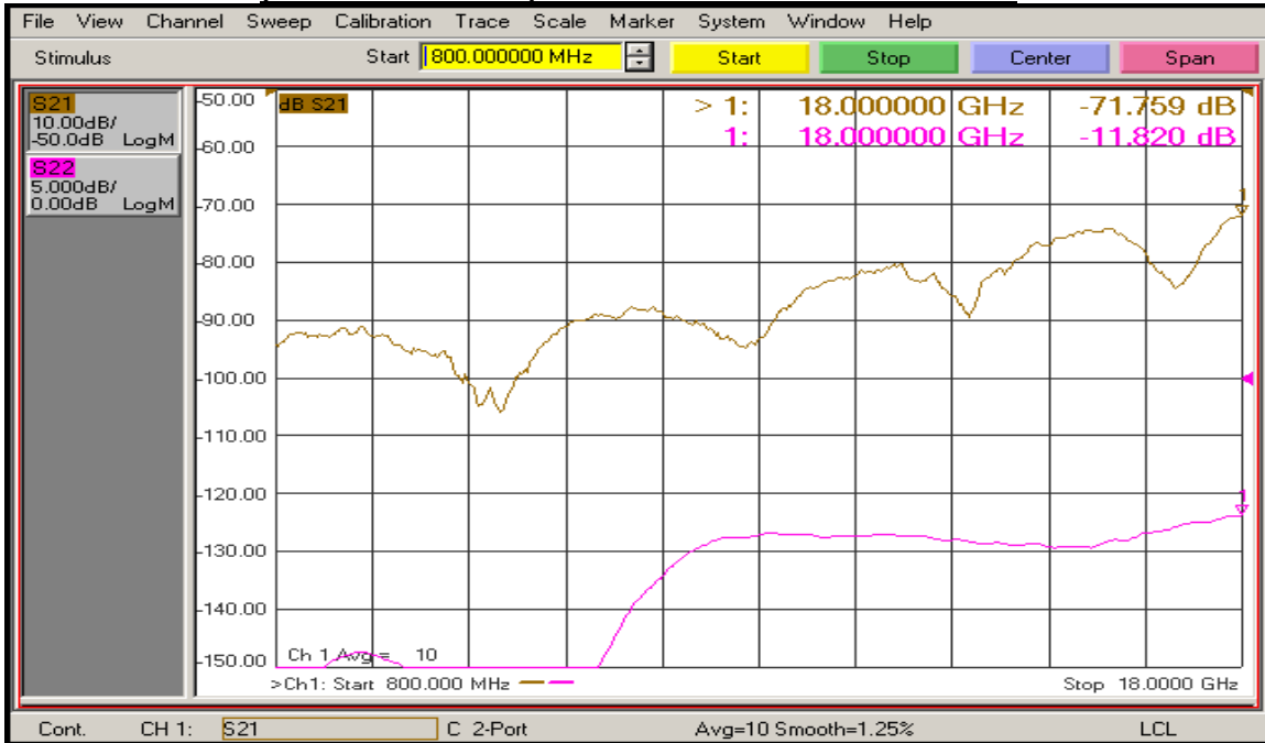
(J8 – J4 with J5 ON) Isolation and Return Loss @ 25°C
