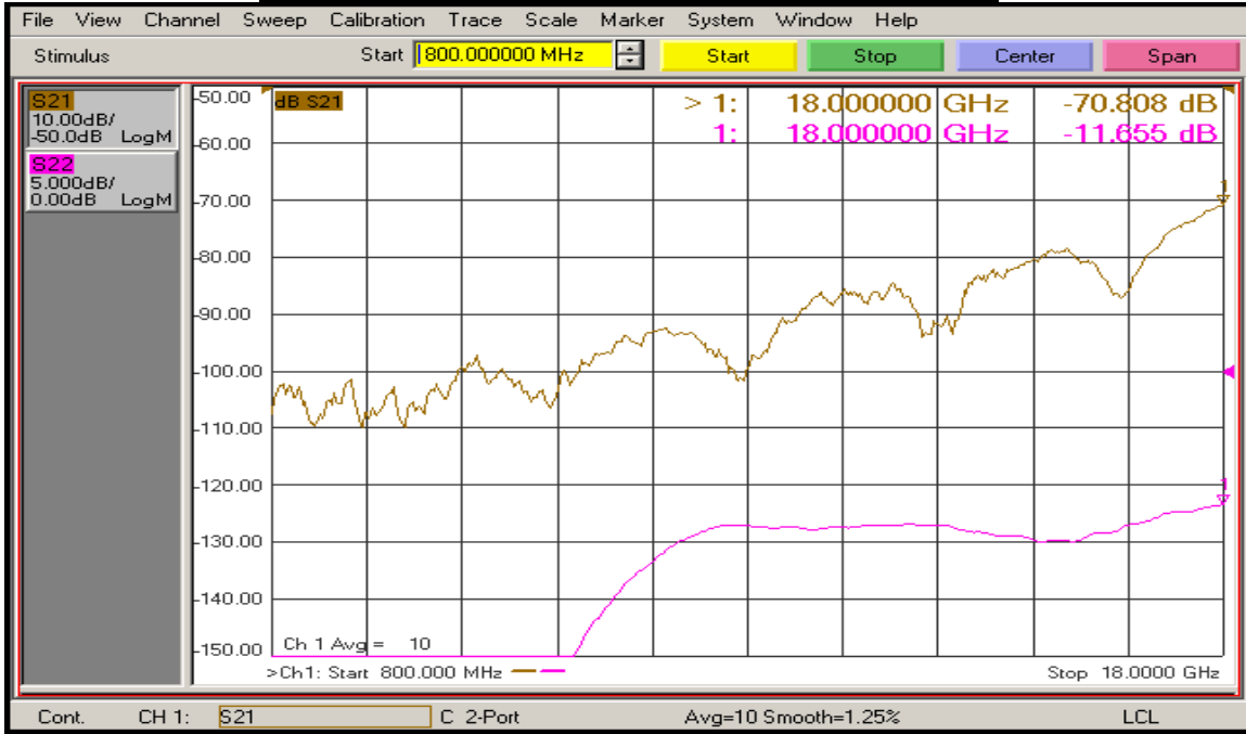
(J8 - J1 with J5 ON) Isolation and Return Loss @ 25°C
