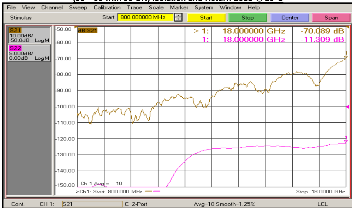
(J8 – J5 with J3 ON) Isolation and Return Loss @ 25°C
