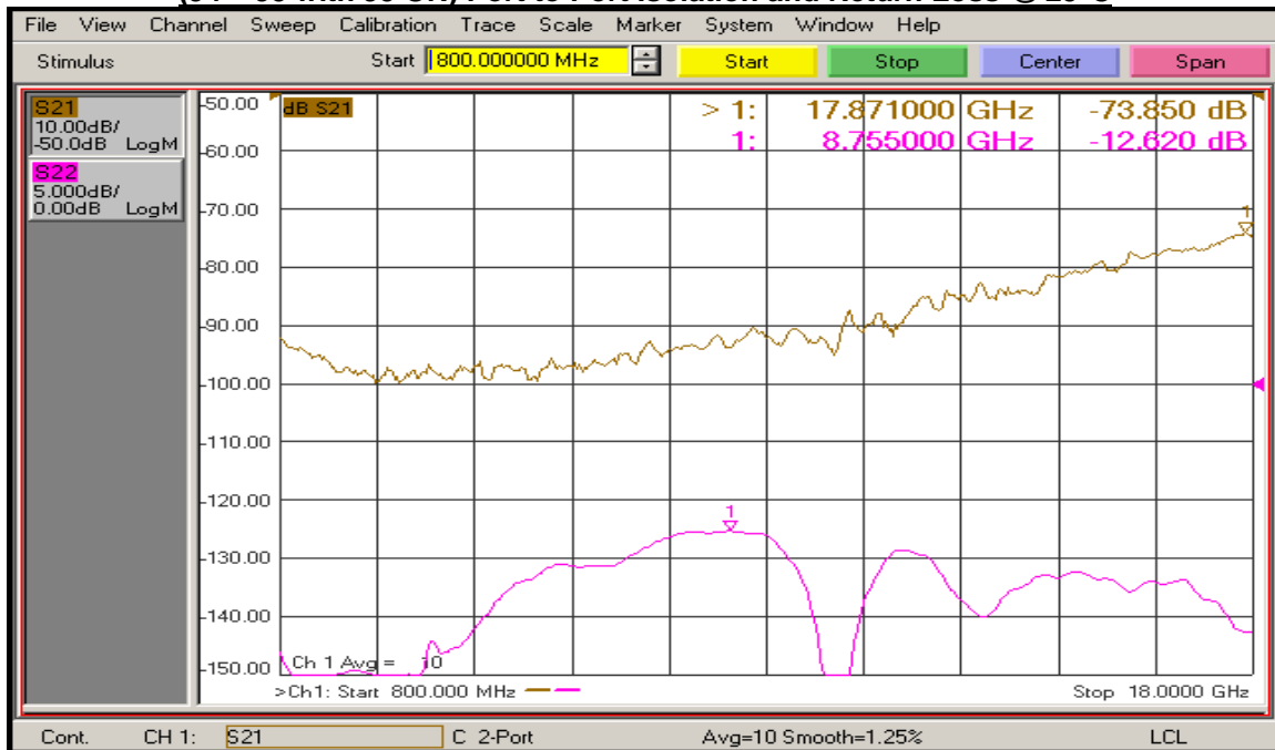
(J4 – J5 with J5 ON) Port to Port Isolation and Return Loss @ 25°C
