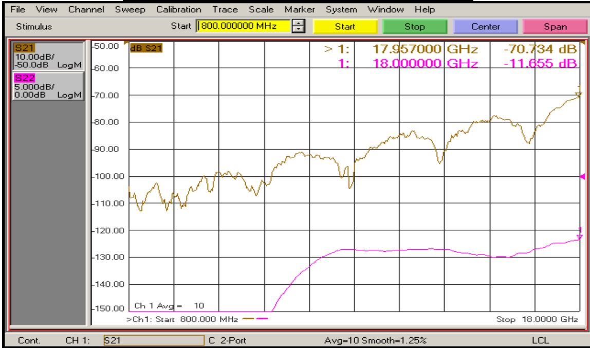
(J8 - J1 with J3 ON) Isolation and Return Loss @ 25°C
