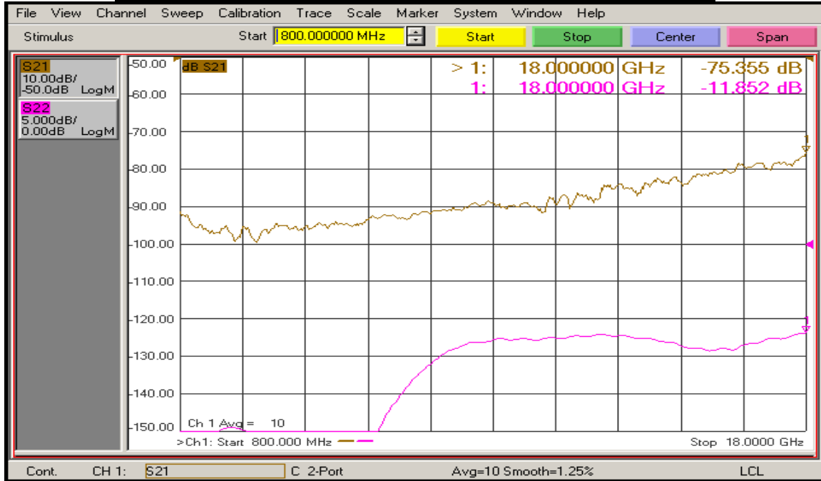
(J6 – J7 with J6 ON) Port to Port Isolation and Return Loss @ 25°C
