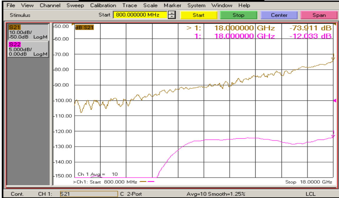
(J8 – J7 All Off) Isolation and Return Loss @ 25°C
