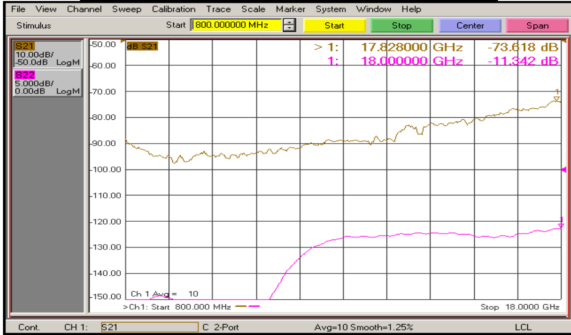
(J4 – J5 with J4 ON) Port to Port Isolation and Return Loss @ 25°C
