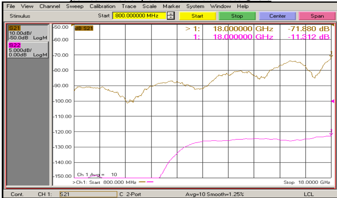
(J8 – J5 with J6 ON) Isolation and Return Loss @ 25°C
