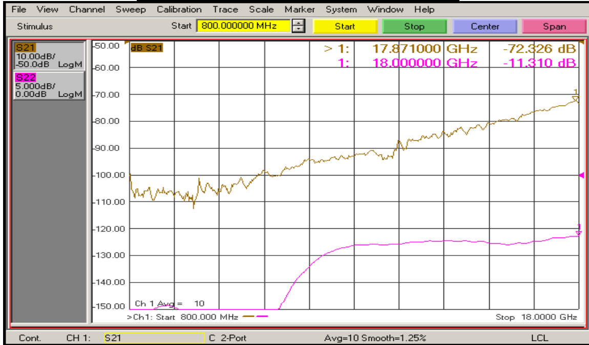
(J8 – J5 All Off) Isolation and Return Loss @ 25°C
