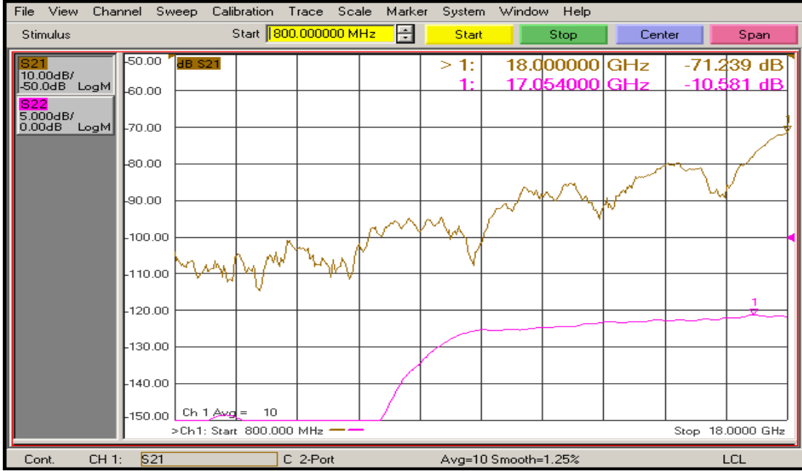
(J8 – J2 with J6 ON) Isolation and Return Loss @ 25°C
