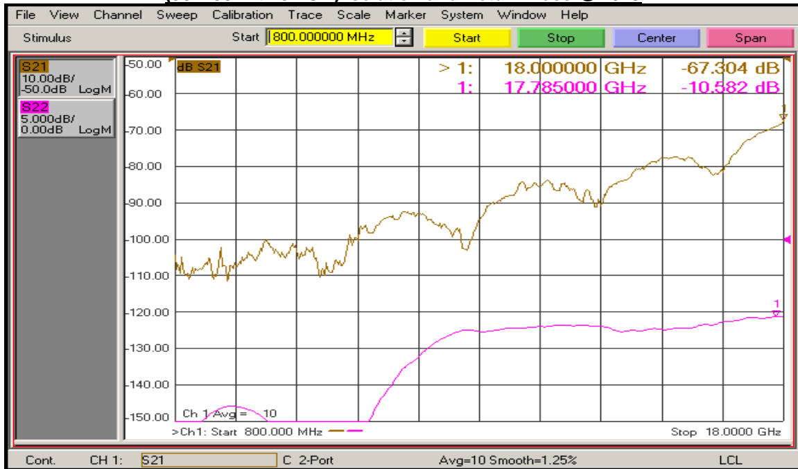
(J8 – J3 with J1 ON) Isolation and Return Loss @ 25°C
