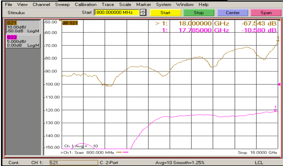
(J8 – J3 with J2 ON) Isolation and Return Loss @ 25°C
