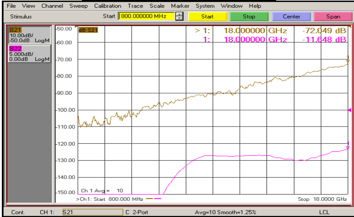
(J8 - J1 All Off ) Isolation and Return Loss @ 25°C
