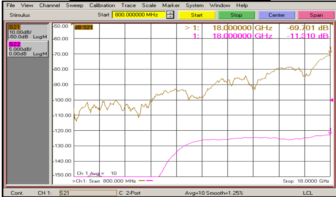
(J8 – J5 with J7 ON) Isolation and Return Loss @ 25°C
