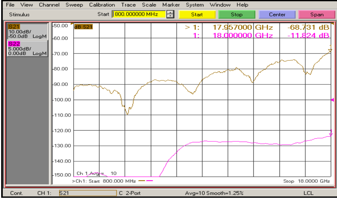
(J8 – J4 with J3 ON) Isolation and Return Loss @ 25°C
