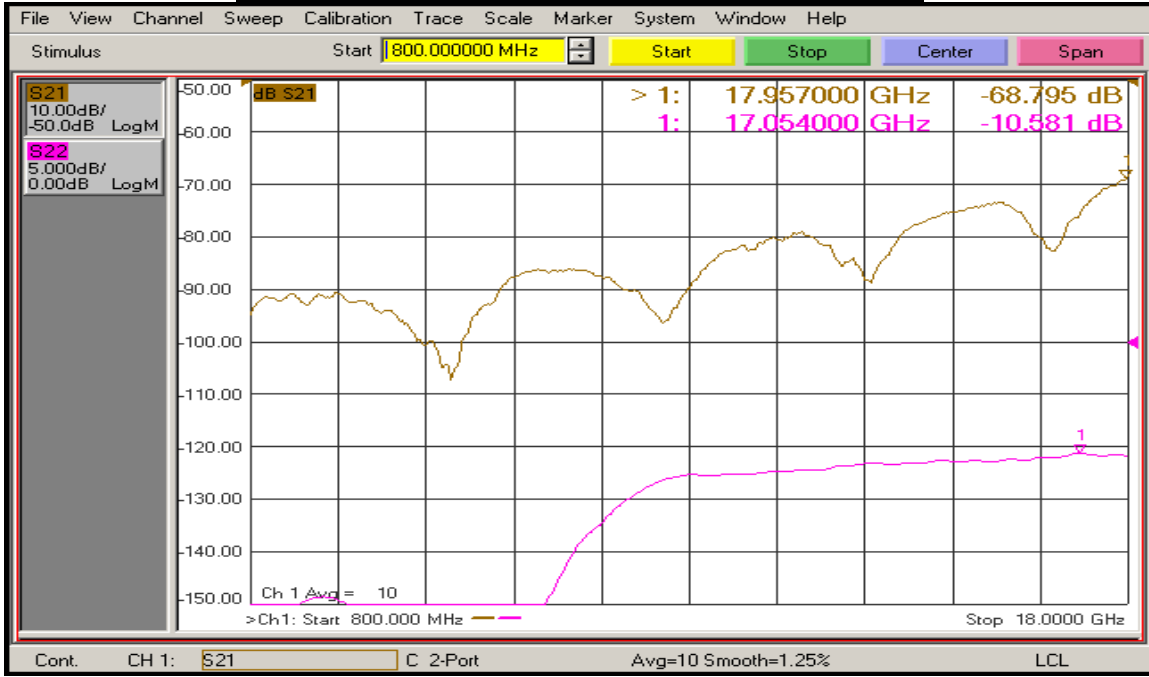
(J8 – J2 with J1 ON) Isolation and Return Loss @ 25°C
