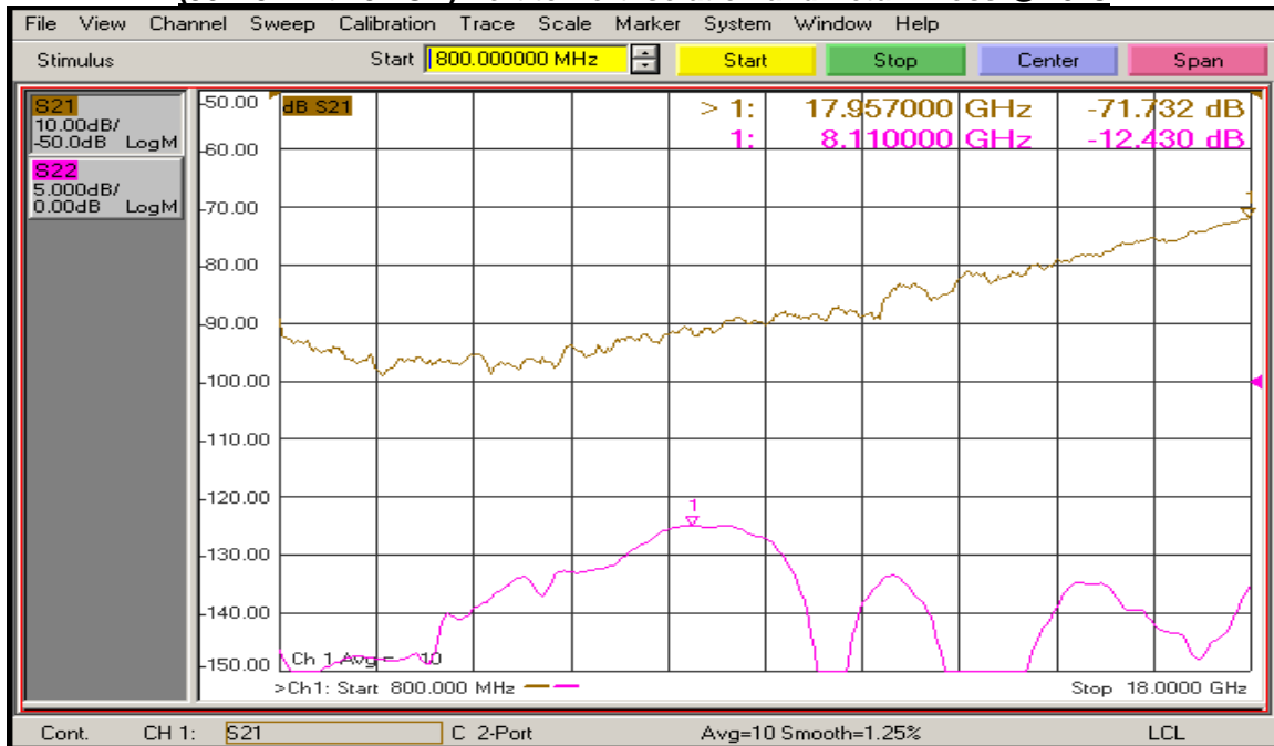
(J3 – J4 with J4 ON) Port to Port Isolation and Return Loss @ 25°C
