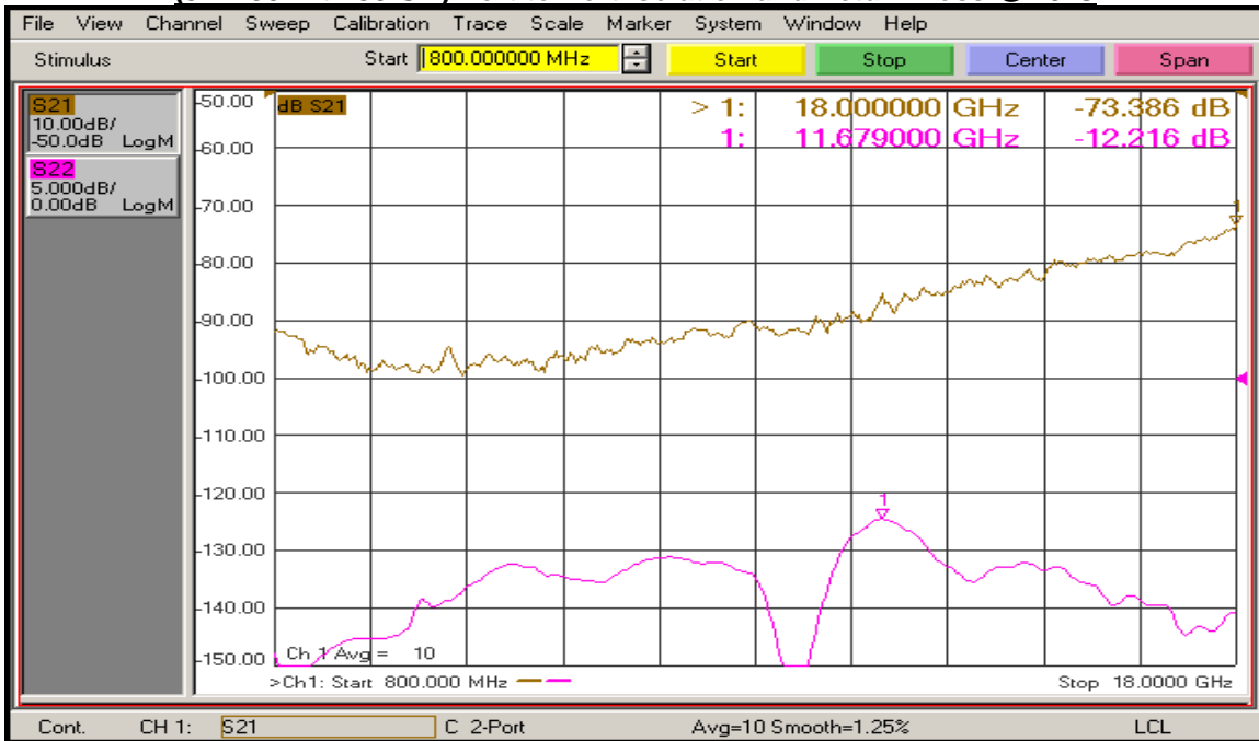
(J2 – J3 with J3 ON) Port to Port Isolation and Return Loss @ 25°C
