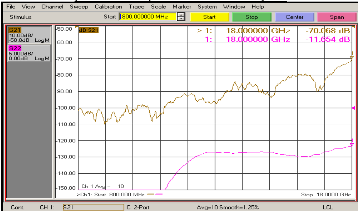
(J8 - J1 with J4 ON) Isolation and Return Loss @ 25°C
