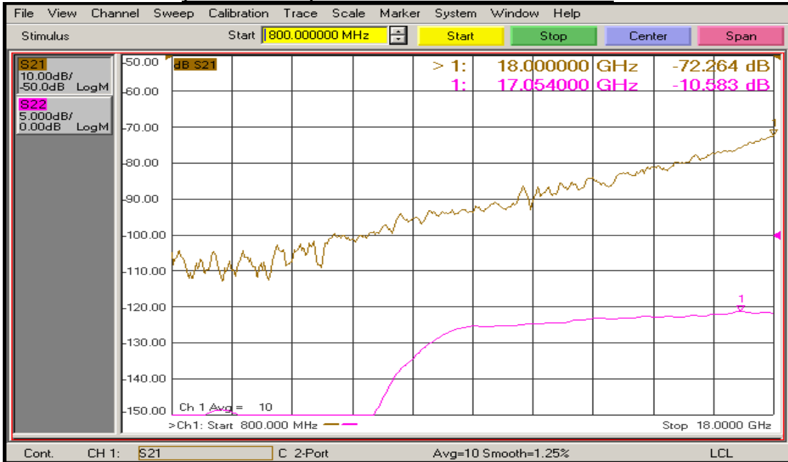
(J8 - J2 All Off) Isolation and Return Loss @ 25°C
