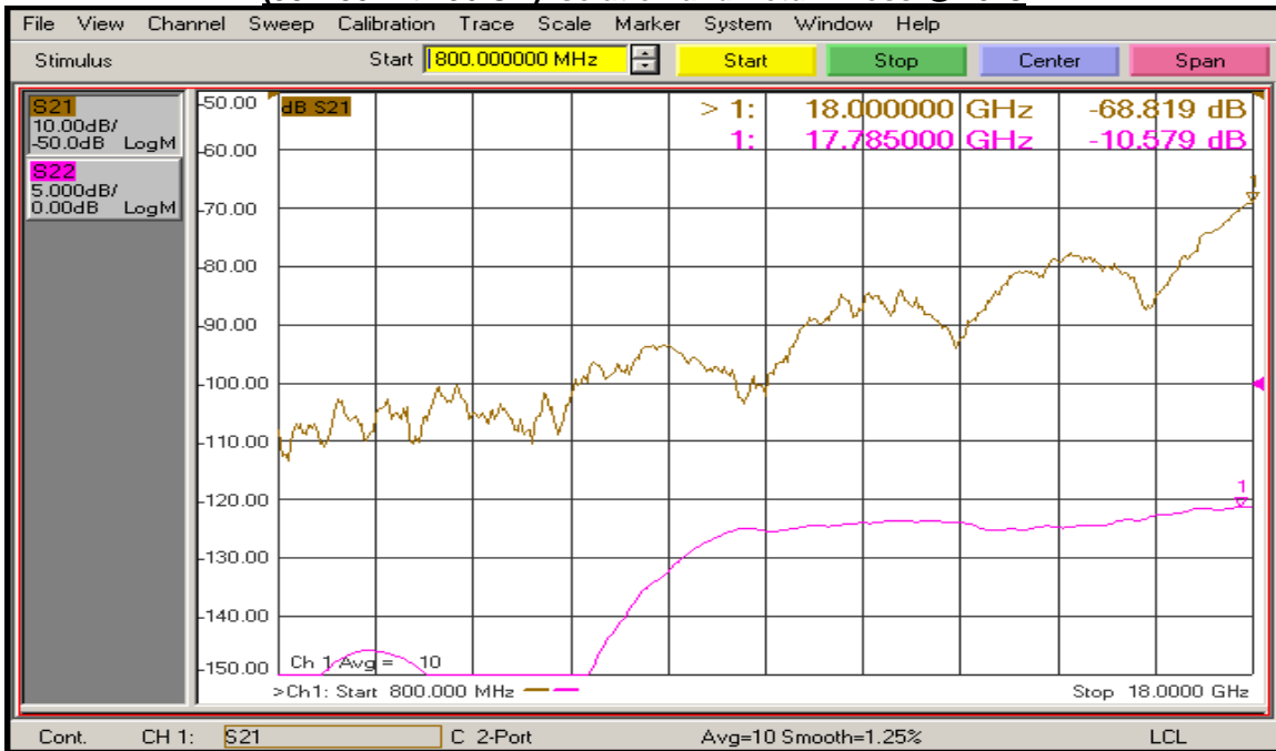
(J8 – J3 with J6 ON) Isolation and Return Loss @ 25°C
