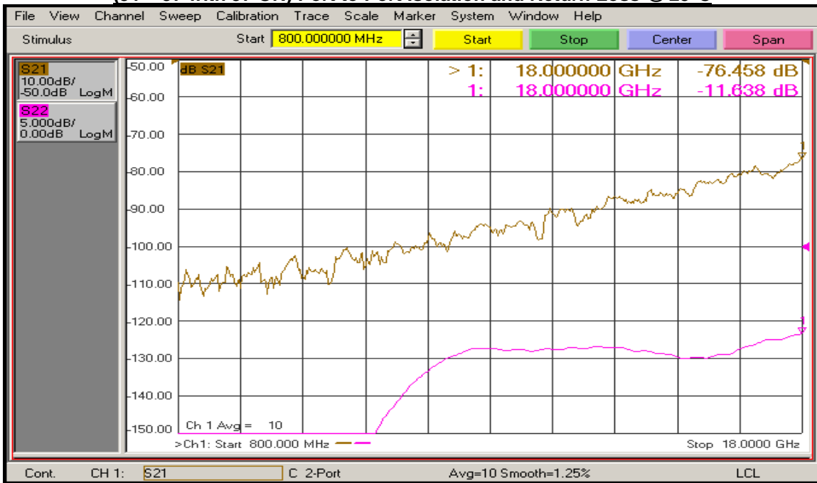
(J1 – J7 with J7 ON) Port to Port Isolation and Return Loss @ 25°C
