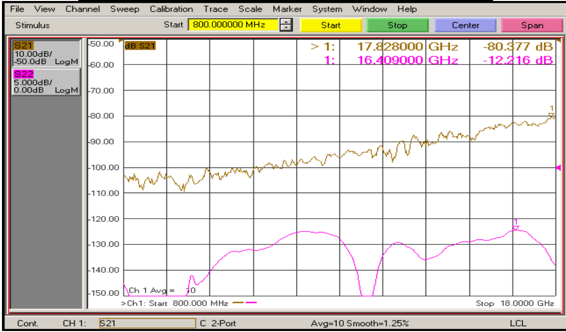
(J1 – J7 with J1 ON) Port to Port Isolation and Return Loss @ 25°C
