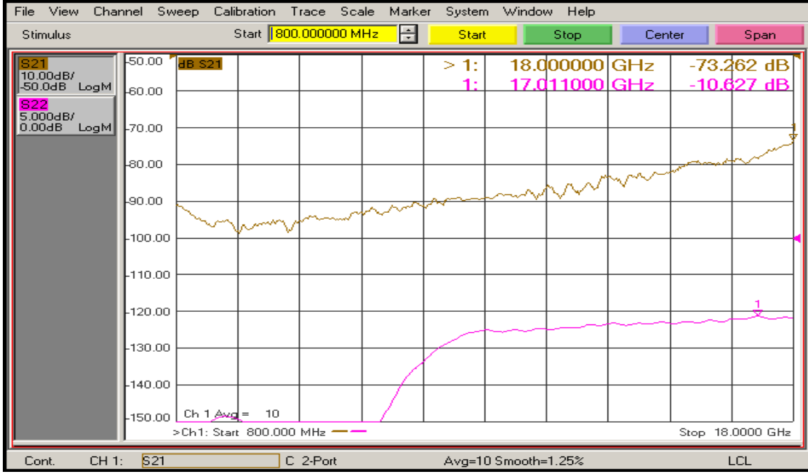
(J1 – J2 with J1 ON) Port to Port Isolation and Return Loss @ 25°C
