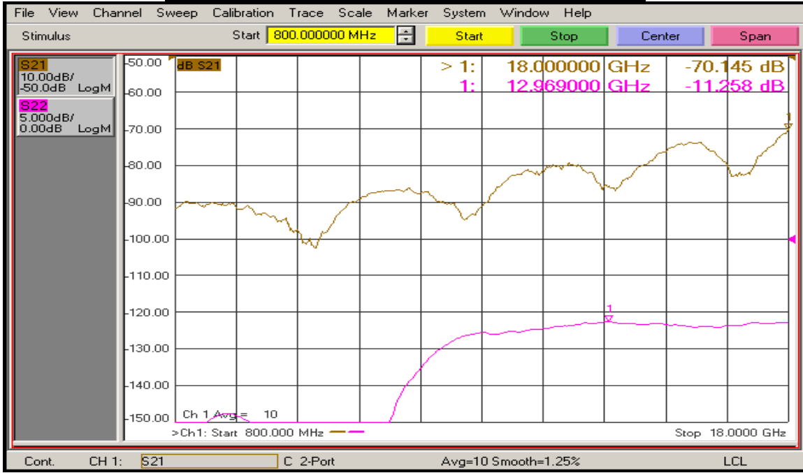
(J8 – J6 with J5 ON) Isolation and Return Loss @ 25°C
