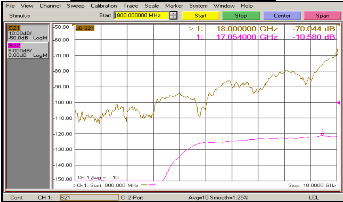
(J8 – J2 with J7 ON) Isolation and Return Loss @ 25°C
