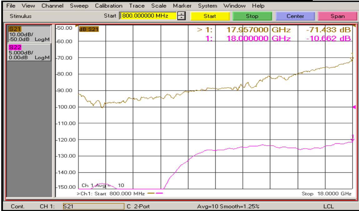
(J2 – J3 with J2 ON) Port to Port Isolation and Return Loss @ 25°C
