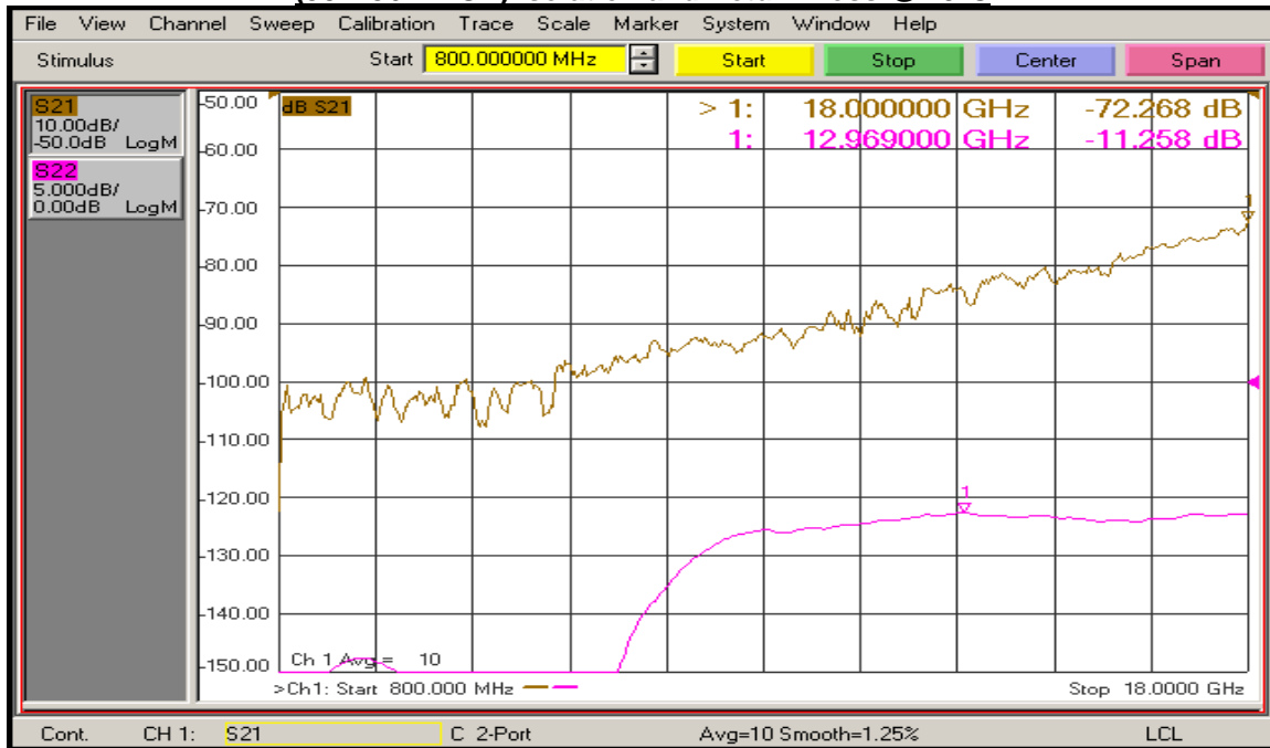
(J8 – J6 All Off) Isolation and Return Loss @ 25°C
