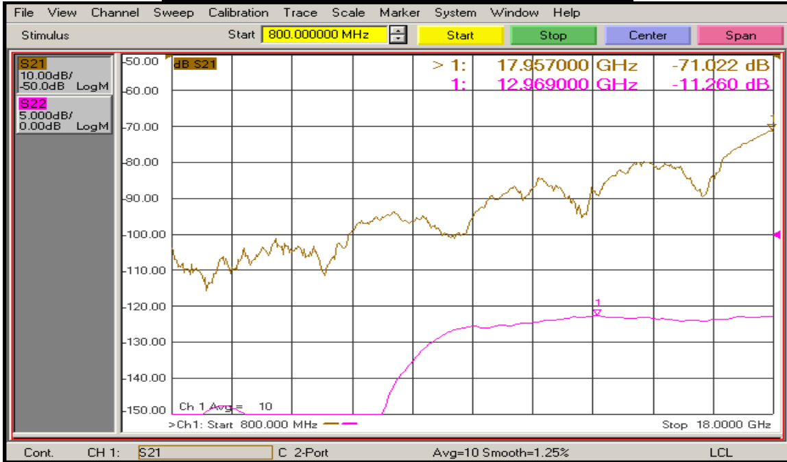
(J8 – J6 with J3 ON) Isolation and Return Loss @ 25°C
