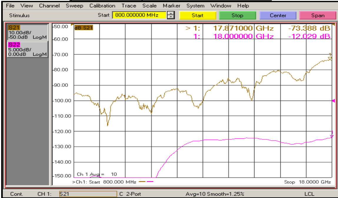
(J8 – J7 with J3 ON) Isolation and Return Loss @ 25°C
