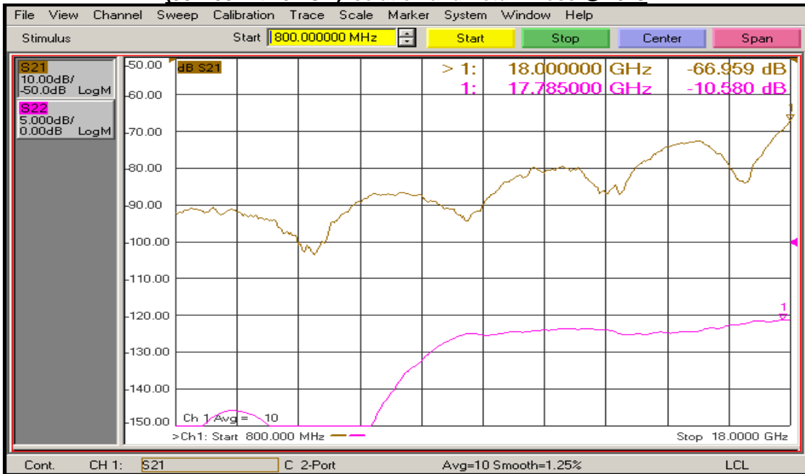
(J8 – J3 with J4 ON) Isolation and Return Loss @ 25°C
