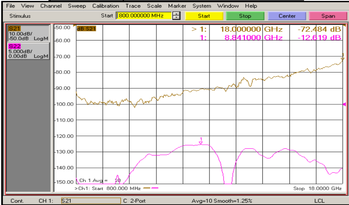
(J1 – J2 with J2 ON) Port to Port Isolation and Return Loss @ 25°C
