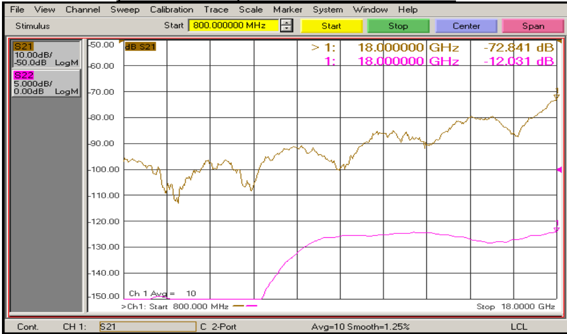
(J8 – J7 with J5 ON) Isolation and Return Loss @ 25°C
