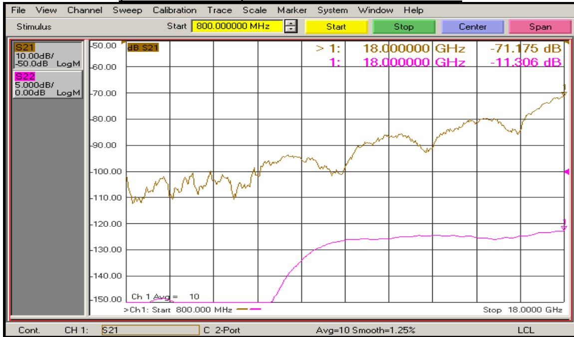
(J8 – J5 with J2 ON) Isolation and Return Loss @ 25°C
