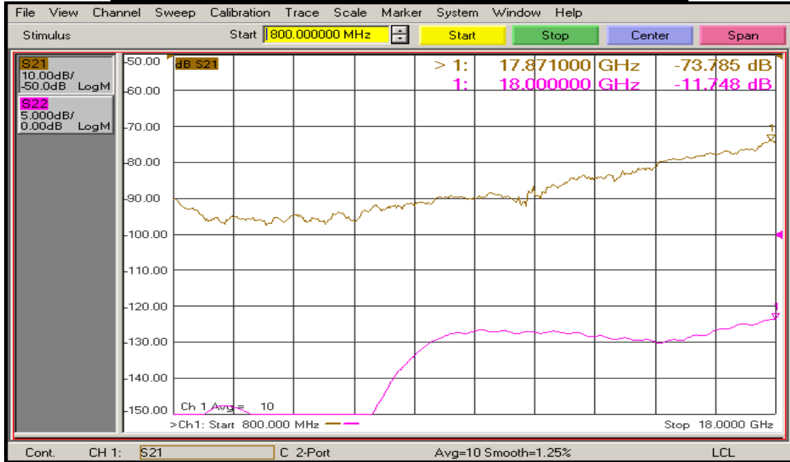
(J3 – J4 with J3 ON) Port to Port Isolation and Return Loss @ 25°C
