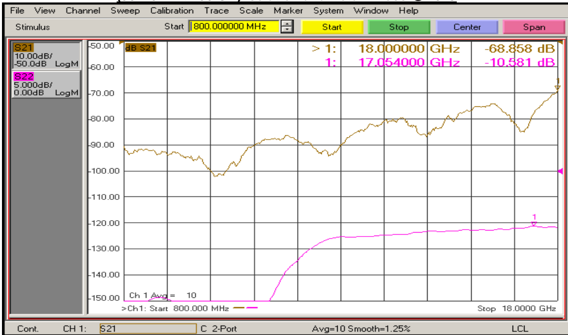
(J8 – J2 with J3 ON) Isolation and Return Loss @ 25°C
