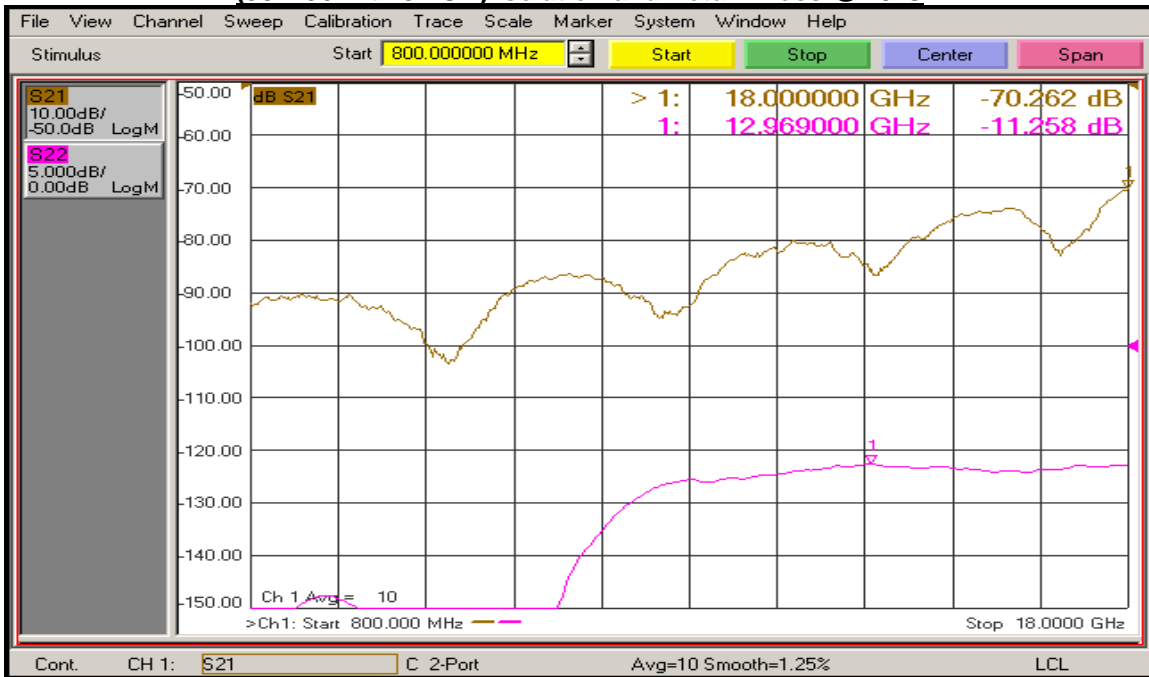
(J8 – J6 with J7 ON) Isolation and Return Loss @ 25°C
