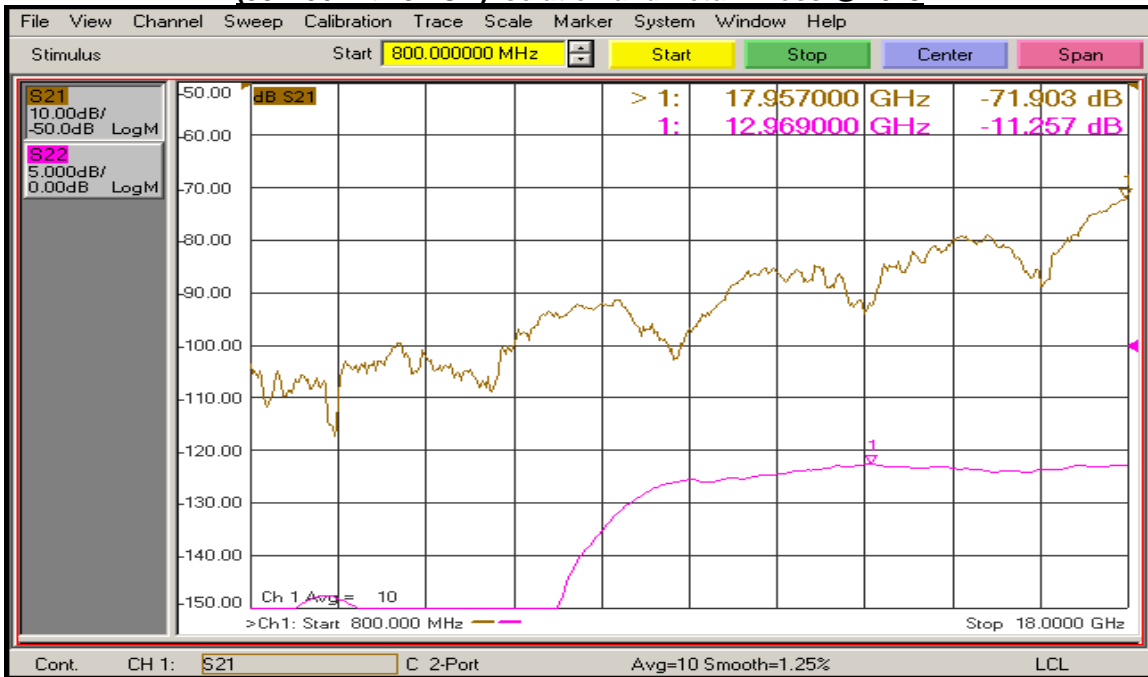
(J8 – J6 with J4 ON) Isolation and Return Loss @ 25°C
