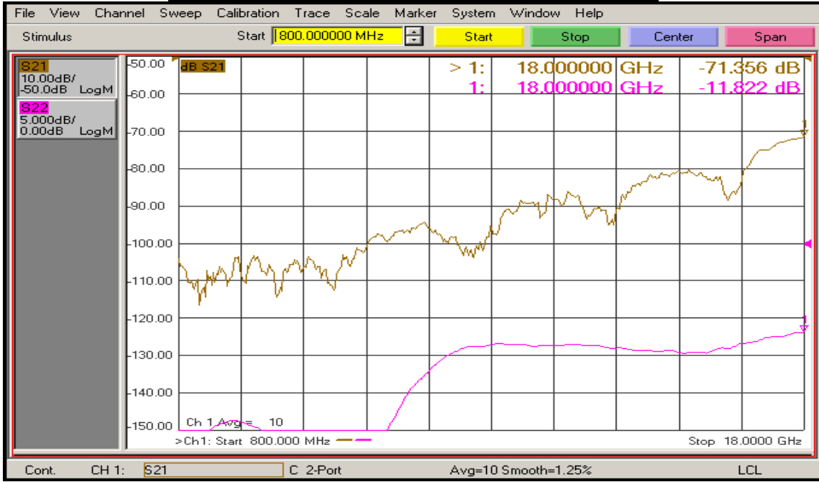
(J8 – J4 with J1 ON) Isolation and Return Loss @ 25°C
