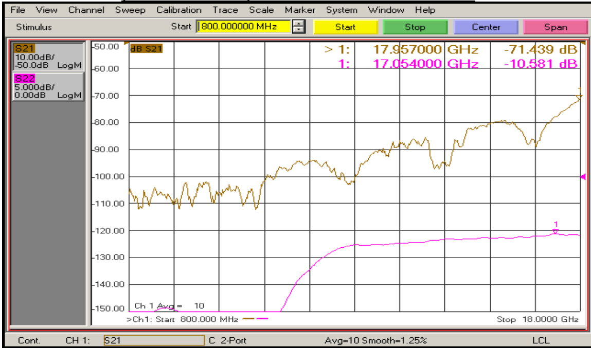
(J8 – J2 with J5 ON) Isolation and Return Loss @ 25°C
