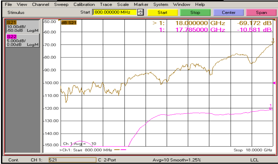
(J8 – J3 with J5 ON) Isolation and Return Loss @ 25°C
