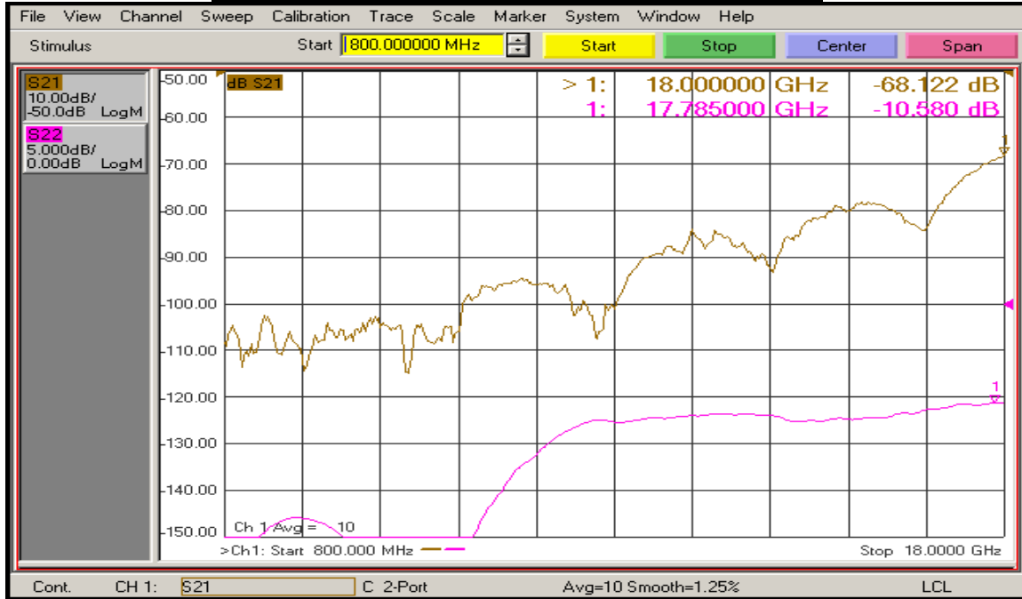
(J8 – J3 with J7 ON) Isolation and Return Loss @ 25°C
