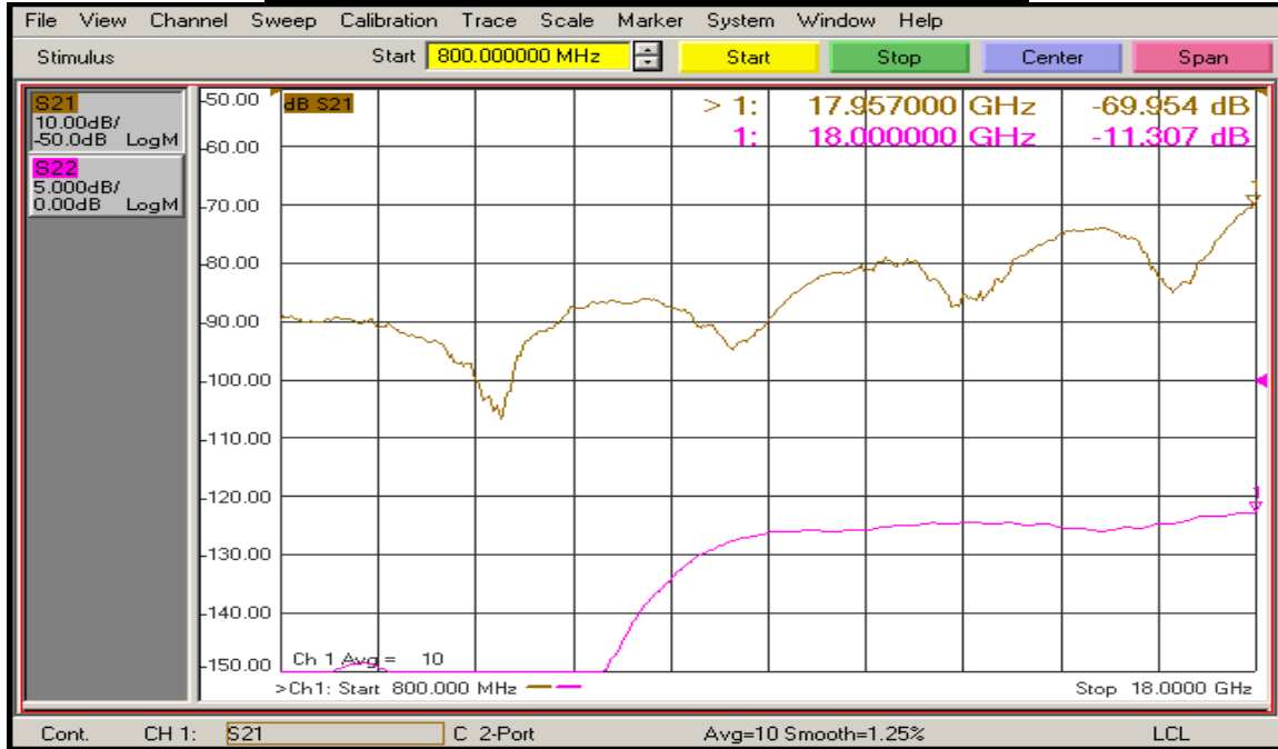
(J8 – J5 with J4 ON) Isolation and Return Loss @ 25°C
