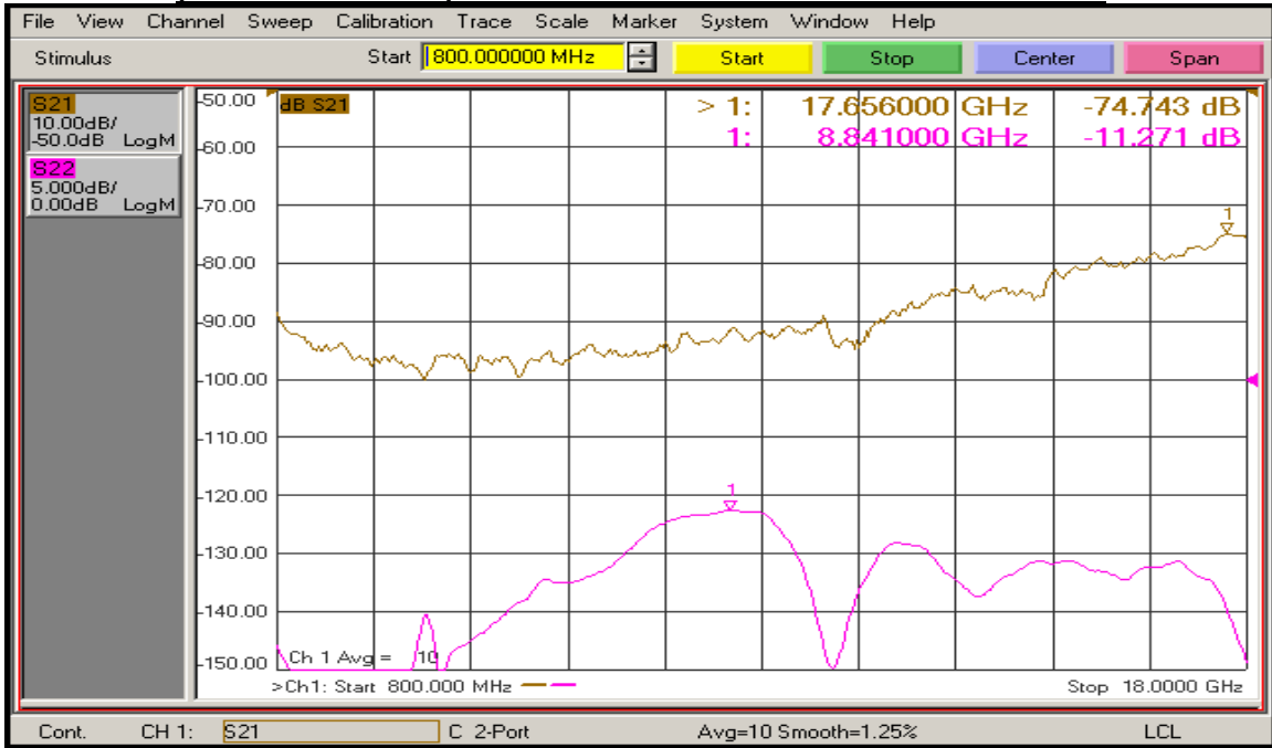
(J5 – J6 with J6 ON) Port to Port Isolation and Return Loss @ 25°C
