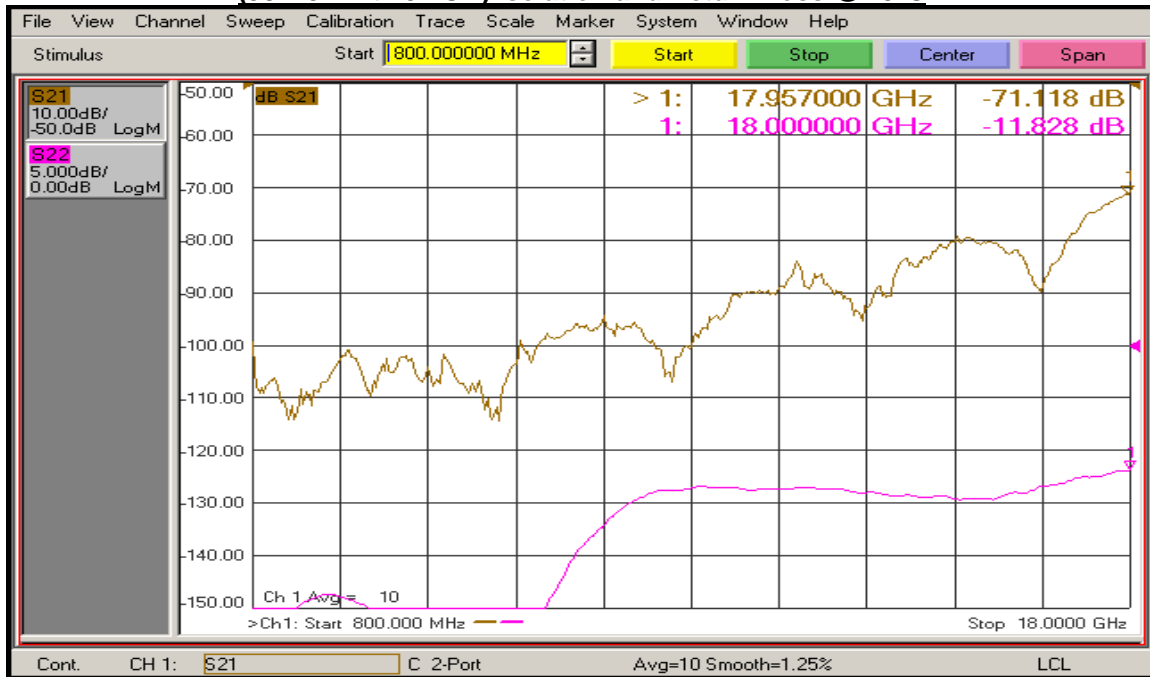
(J8 – J4 with J7 ON) Isolation and Return Loss @ 25°C
