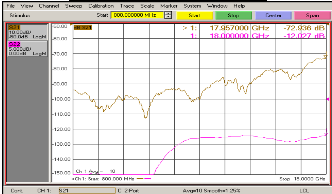
(J8 – J7 with J1 ON) Isolation and Return Loss @ 25°C
