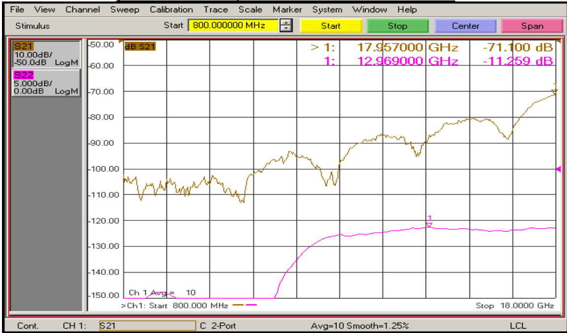
(J8 – J6 with J2 ON) Isolation and Return Loss @ 25°C
