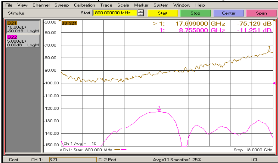
(J6 – J7 with J7 ON) Port to Port Isolation and Return Loss @ 25°C
