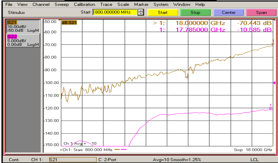
(J8 – J3 All Off) Isolation and Return Loss @ 25°C
