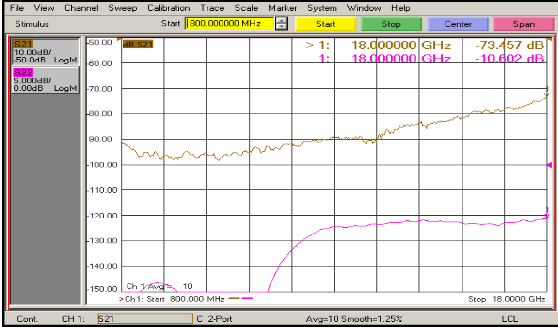
(J5 – J6 with J5 ON) Port to Port Isolation and Return Loss @ 25°C
