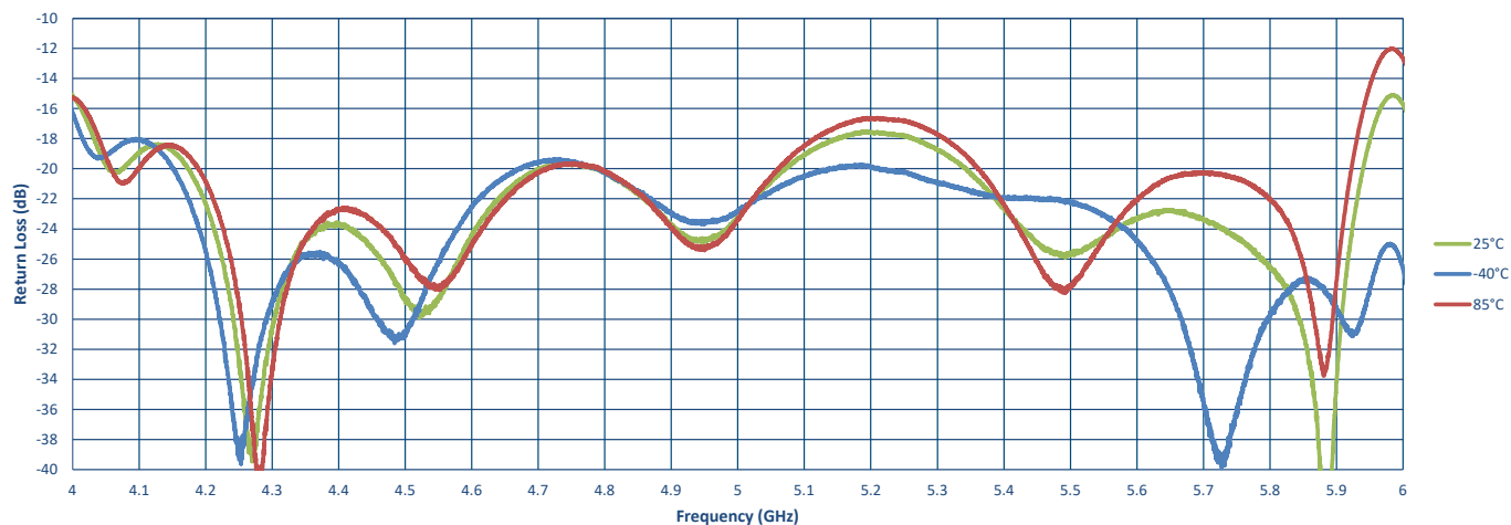
Band 2 - Passband Return Loss - S11
