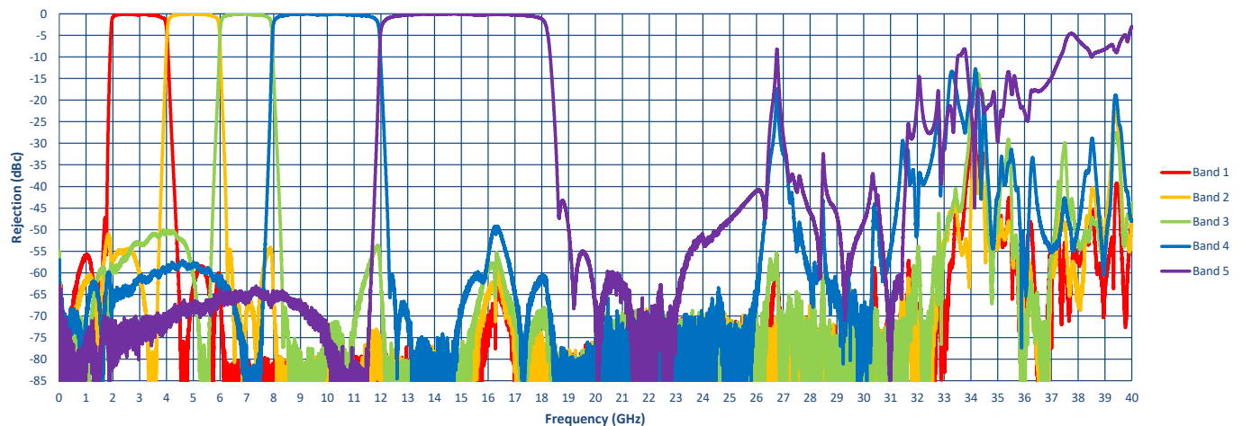
All Bands - Extended (+85°C)
