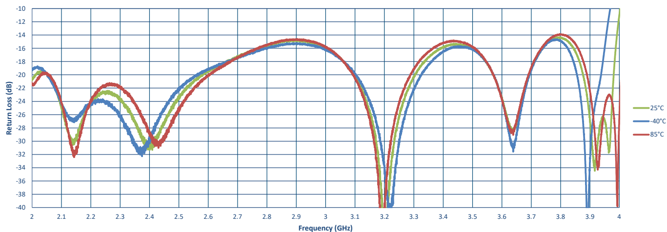
Band 1 - Passband Return Loss - S22
