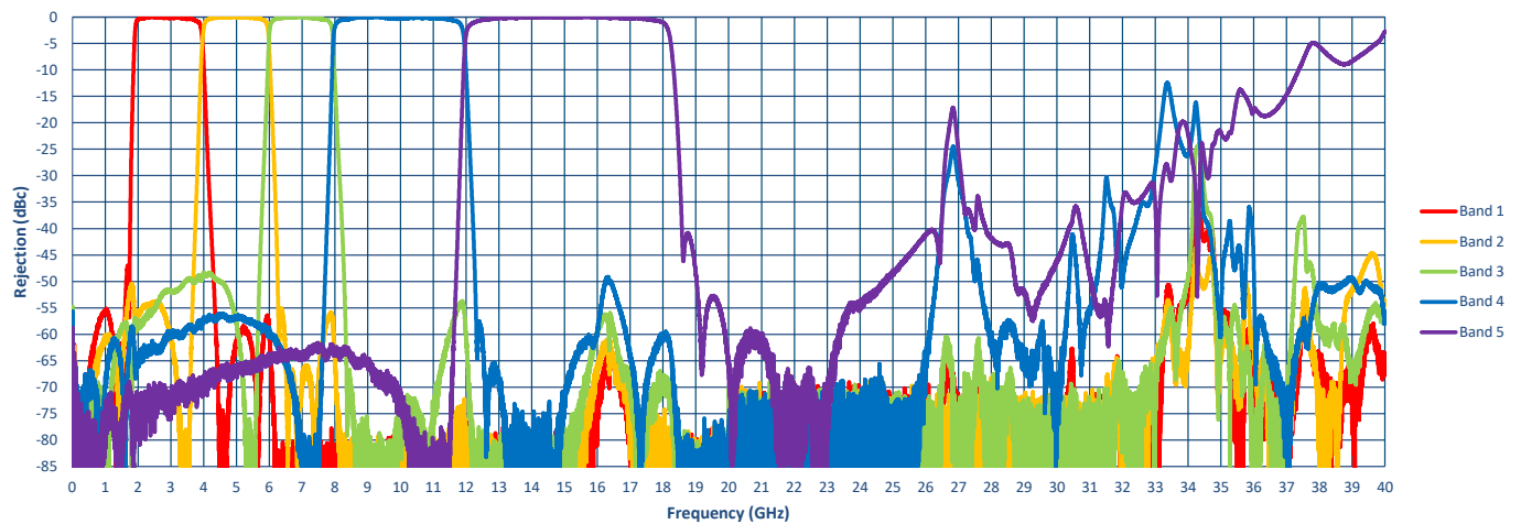
All Bands - Extended (-40°C)
