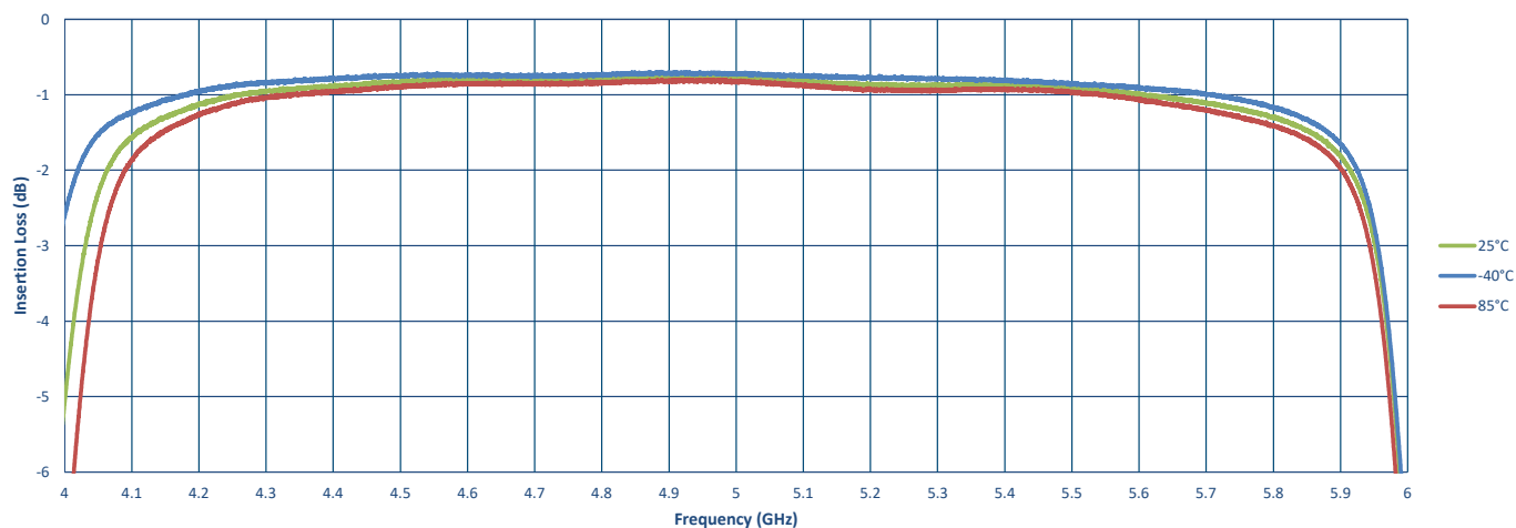
Band 2 - Passband Insertion Loss
