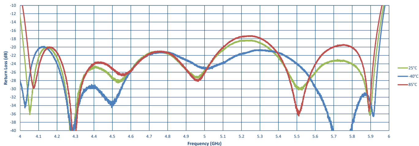
Band 2 - Passband Return Loss - S22
