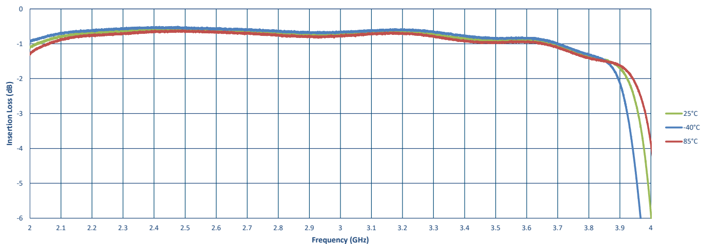
Band 1 - Passband Insertion Loss
