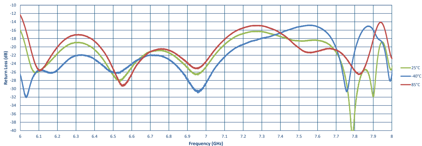
Band 3 - Passband Return Loss - S11
