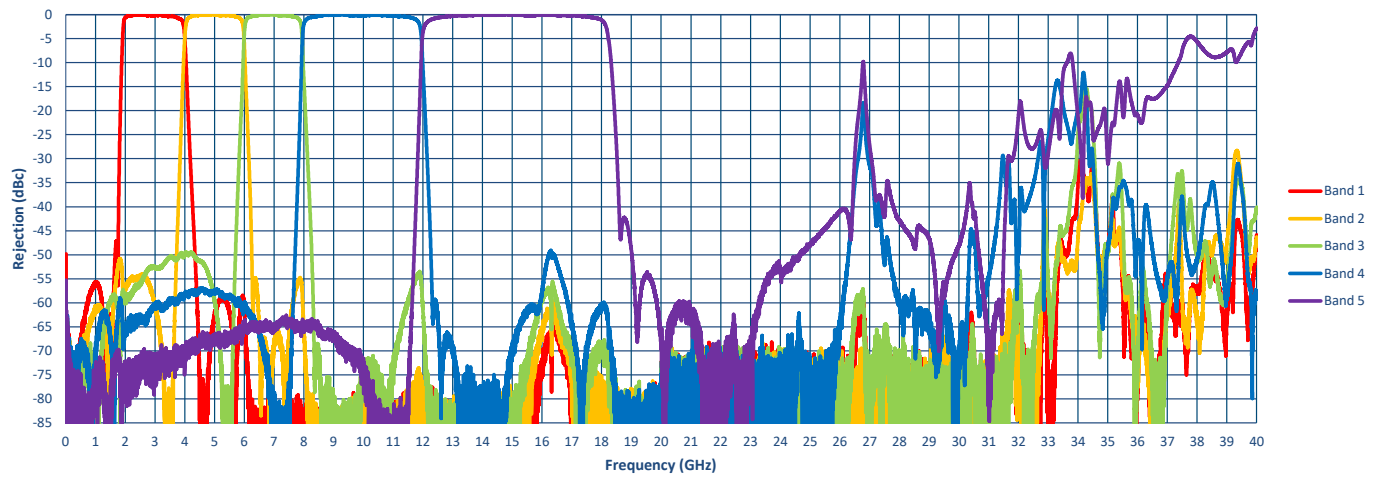
All Bands - Extended (+25°C)
