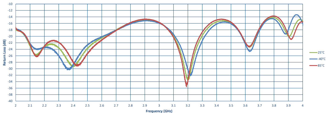
Band 1 - Passband Return Loss - S11
