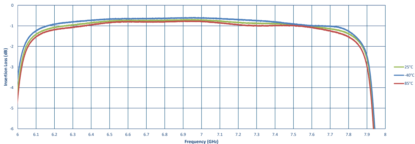
Band 3 - Passband Insertion Loss
