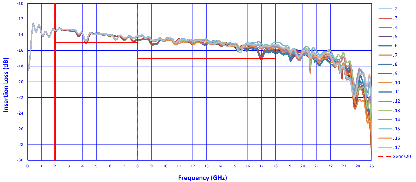
Absolute Insertion Loss (+85°C)
