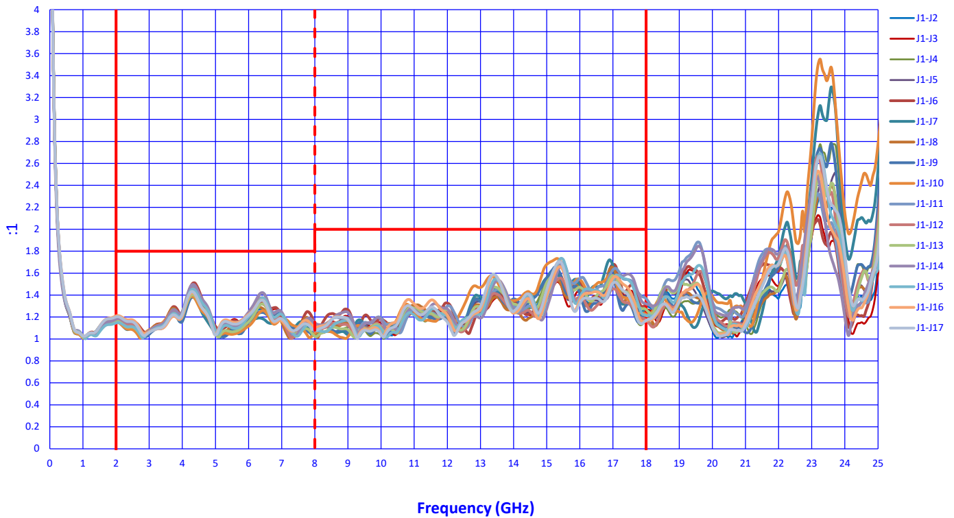
VSWR OUT (+85°C)
