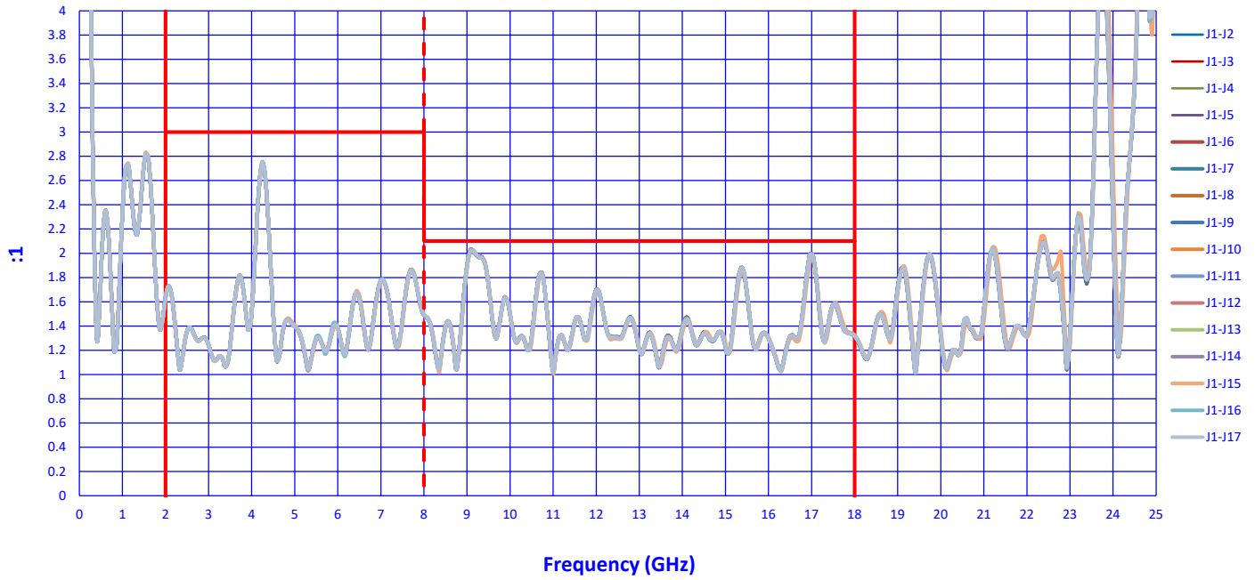
VSWR IN (+85°C)
