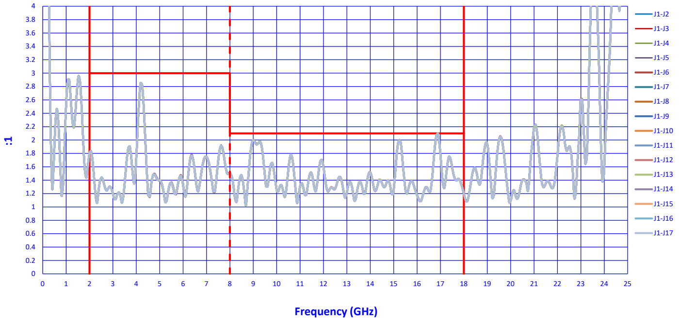
VSWR IN (-55°C)
