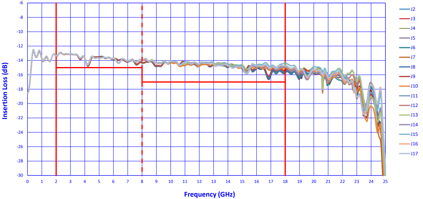
Absolute Insertion Loss (-55°C)
