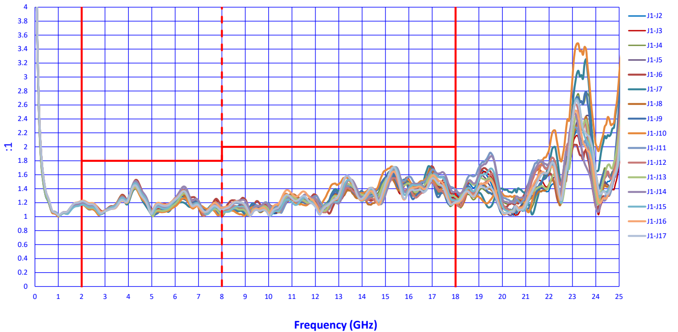
VSWR OUT (+25°C)
