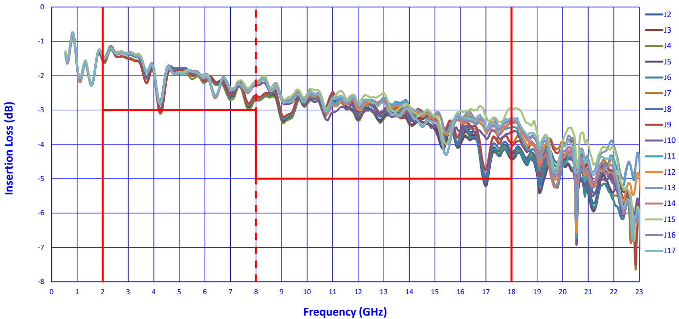
Insertion Loss over Theoretical Power Split of 12 dB (+85°C)
