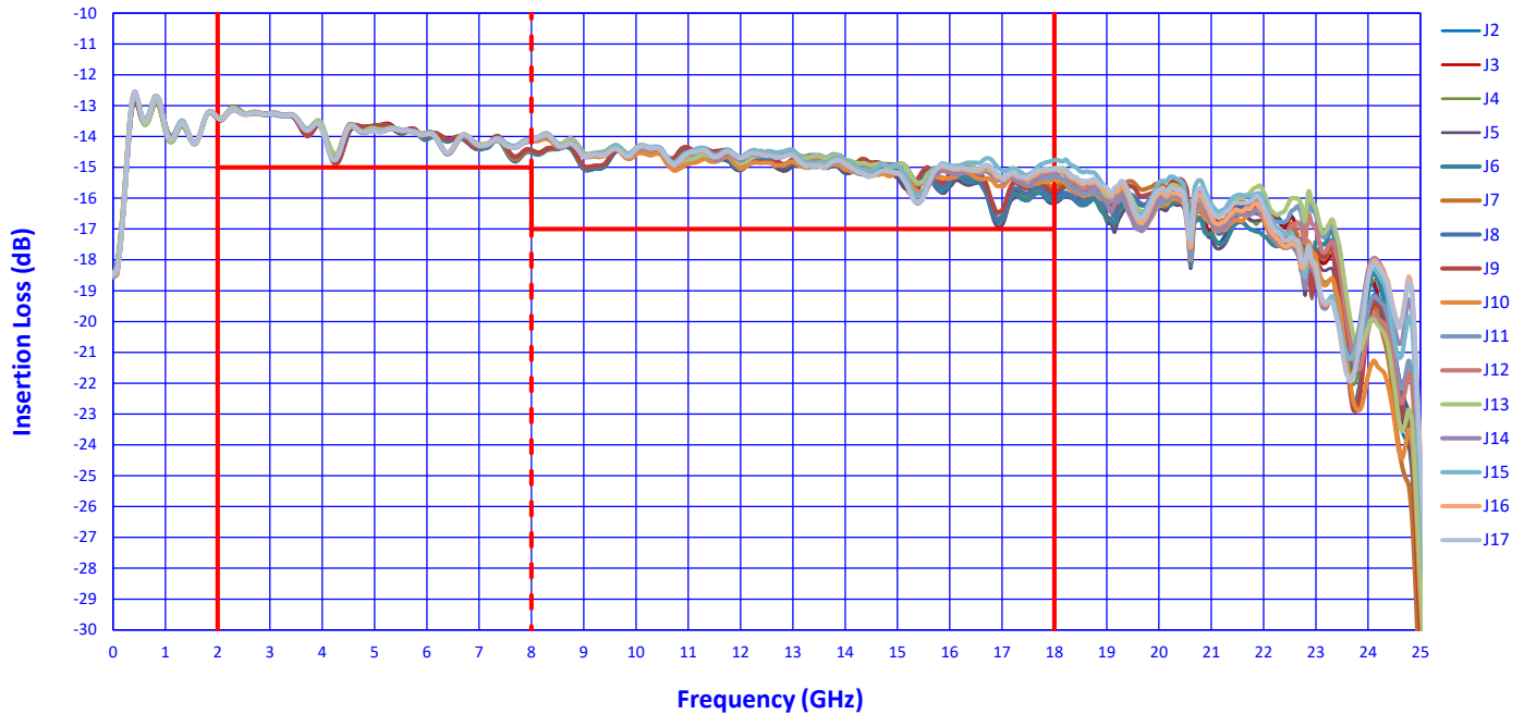
Absolute Insertion Loss (+25°C)
