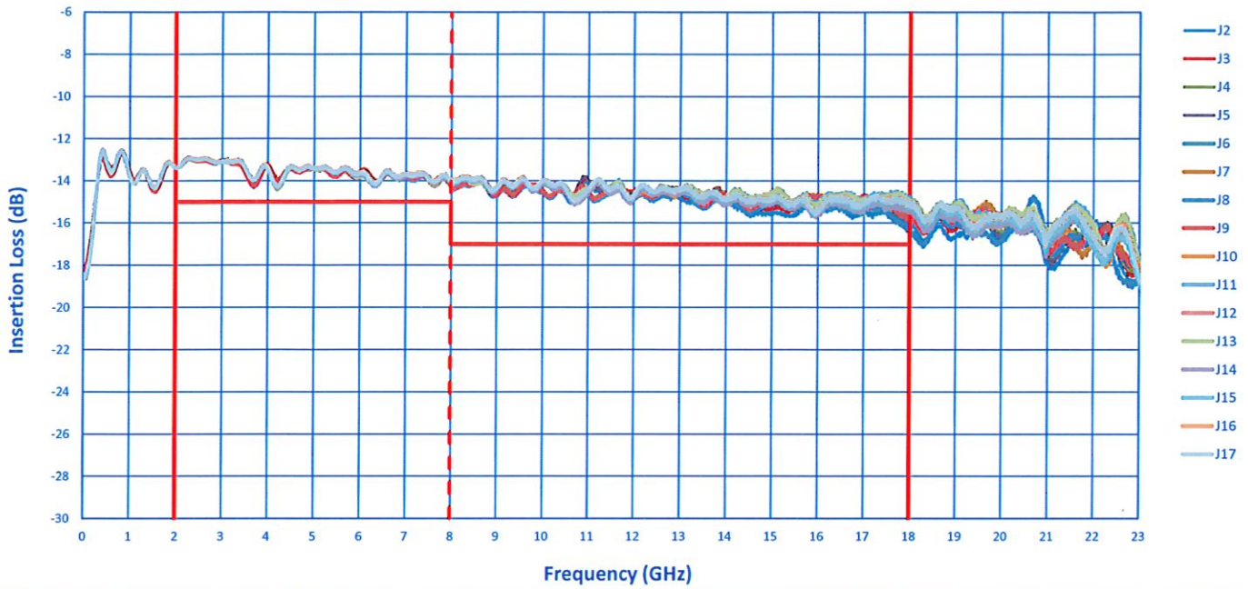
Absolute Insertion Loss (-55°C)
