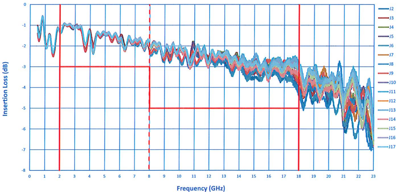
Insertion Loss over Theoretical Power Split of 12 dB (-55°C)
