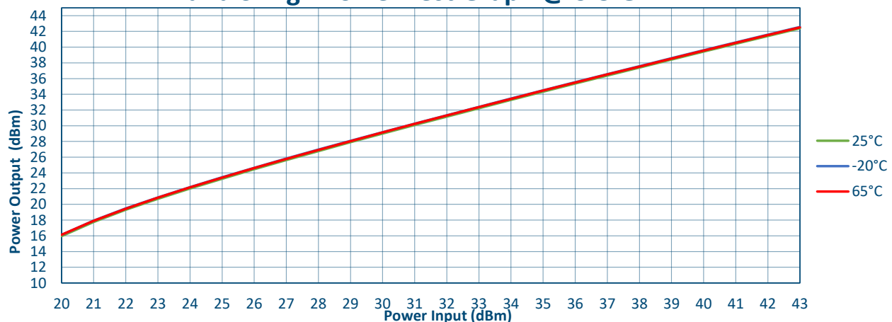
Band 3 High Power Test Graph @ 9.5 GHz
