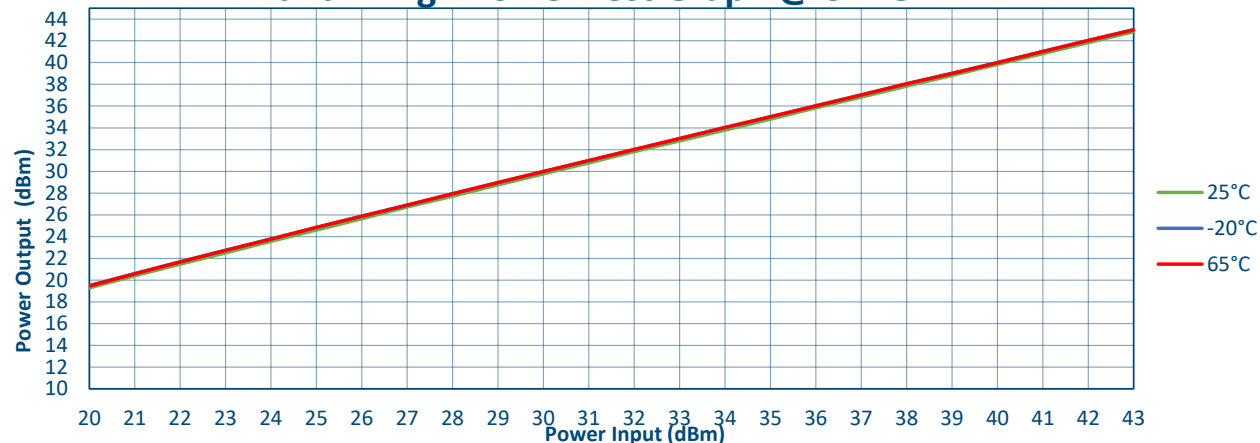
Band 2 High Power Test Graph @ 5.7 GHz
