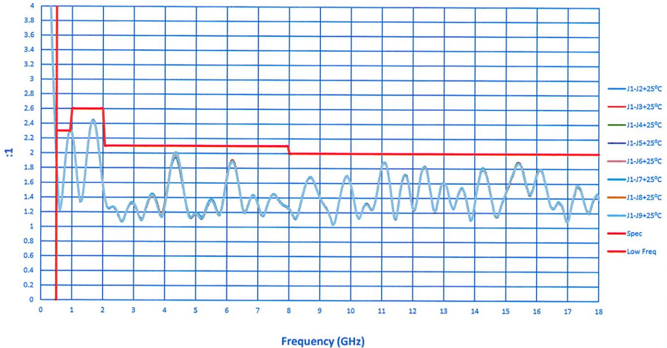
VSWR IN (+25°C)
