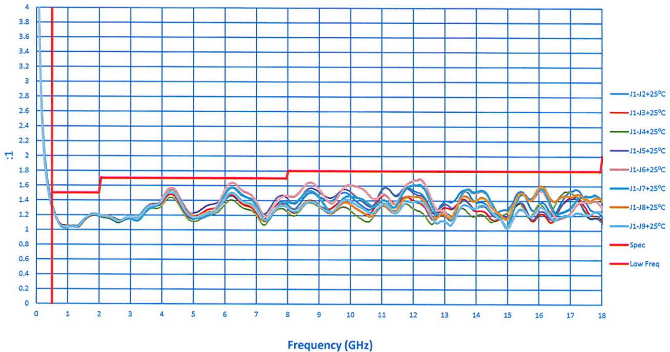
VSWR OUT (+25°C)
