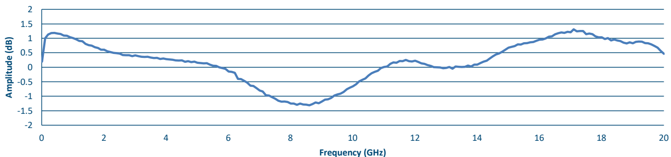
Gain Flatness
