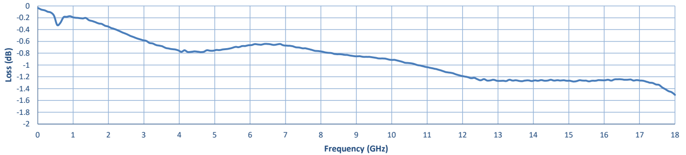
Insertion Loss
