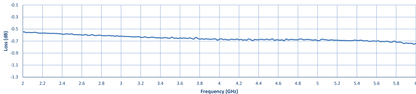
Insertion Loss
