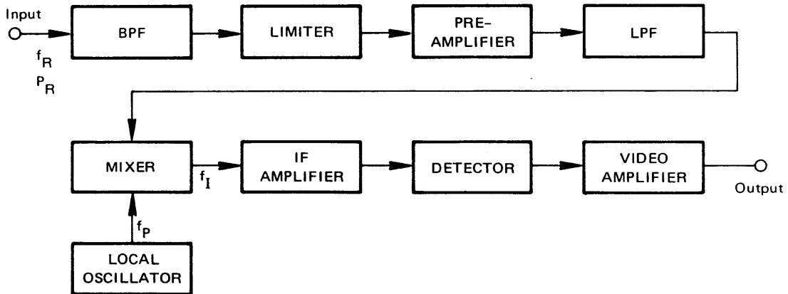
FIGURE IV-3 COMPLEX AM RECEIVER CONCEPT
