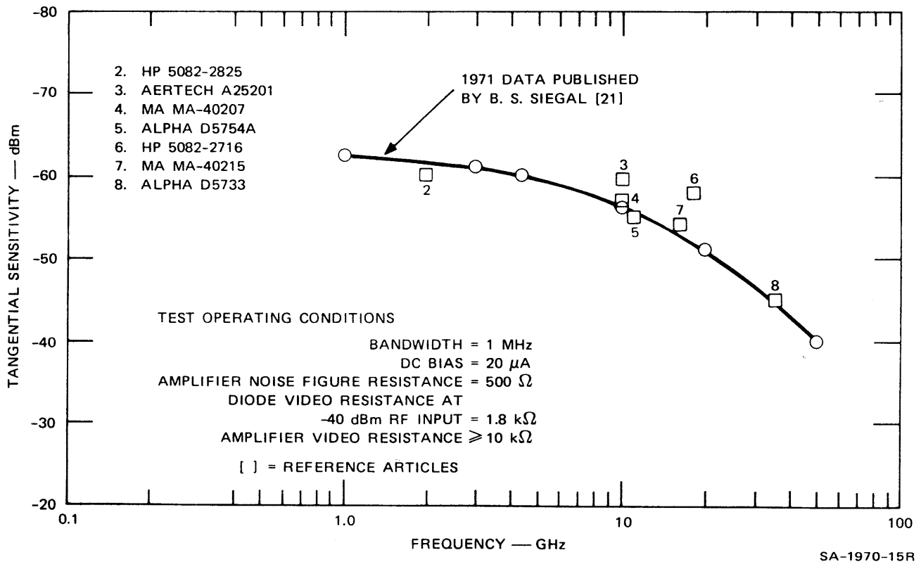
FIGURE VI-7 TANGENTIAL SENSITIVITY PERFORMANCE OF COMMERCIAL SILICON SCHOTTKY BARRIER DETECTOR DIODES — 1973
