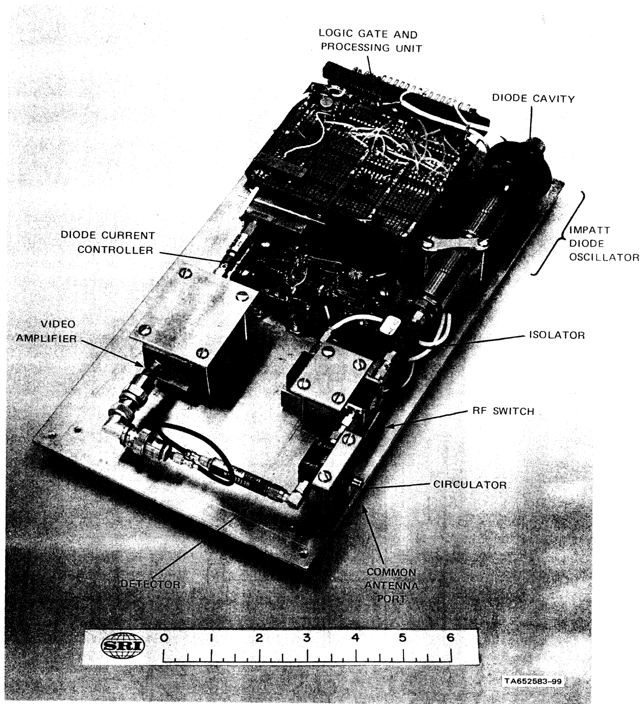
FIGURE V-13 14.5-GHz SOLID-STATE COOPERATIVE BEACON TRANSPONDER FOR AIRPORT SURFACE DETECTION (ASD) RADAR
