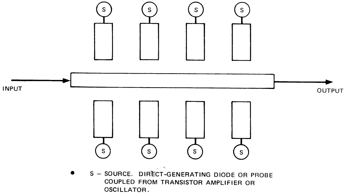
FIGURE VII-8 ITERATIVE POWER-COMBINER SCHEME FOR AMPLIFIERS AND OSCILLATORS
