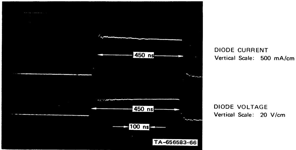
FIGURE V-22 IMPATT DIODE OSCILLATOR CURRENT AND VOLTAGE RESPONSE
