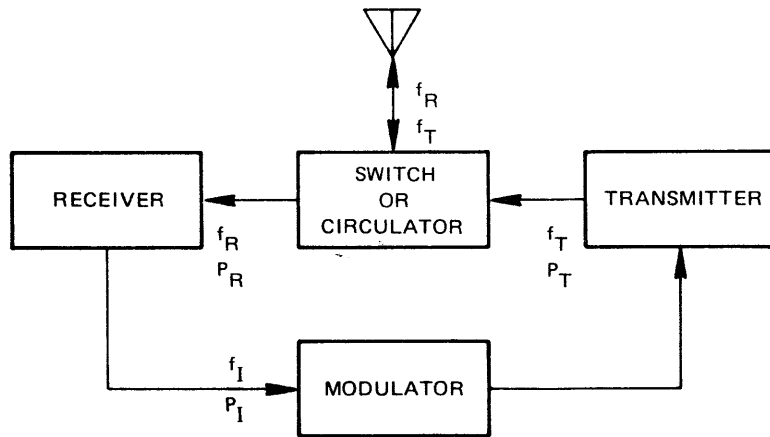
(b) ONE-ANTENNA TRANSPONDER
