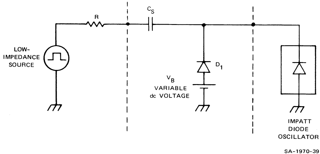
FIGURE V-8 PULSE-ADDING BIAS CIRCUIT FOR IMPATT DIODE OSCILLATOR
