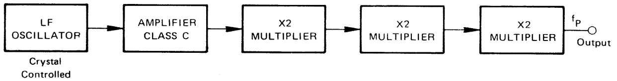
(a) CRYSTAL-CONTROLLED OSCILLATOR/VARACTOR MULTIPLIER COMBINATION
