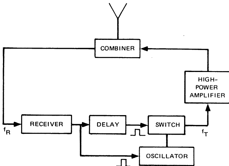
FIGURE VII-14 HIGH-POWER BEACON TRANSPONDER
