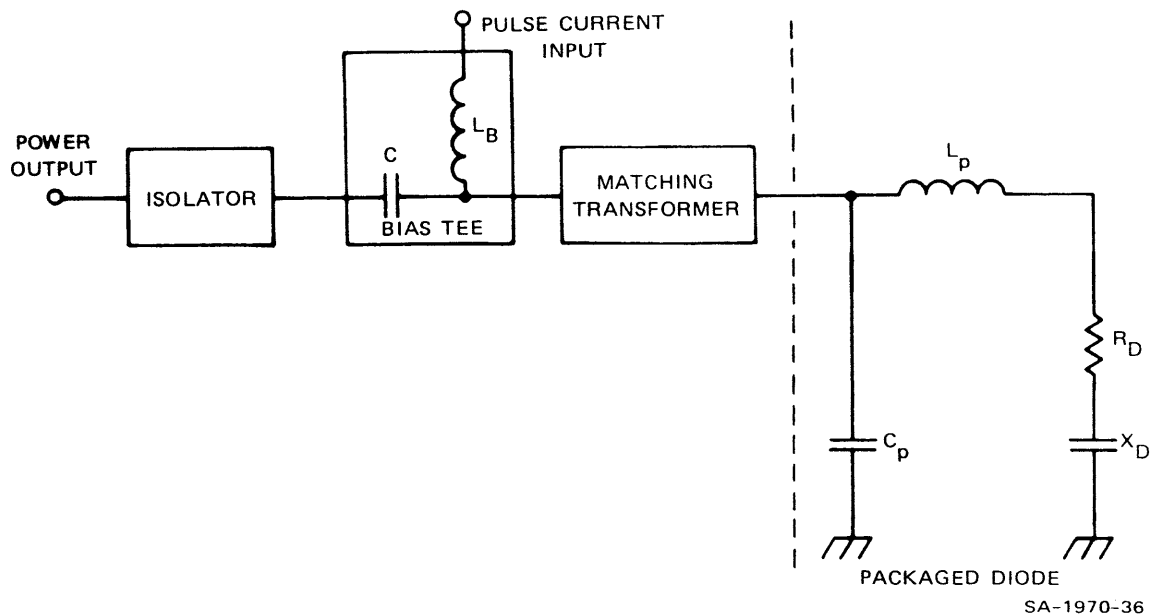
FIGURE V-4 CIRCUIT SCHEMATIC OF LOW-Q COAXIAL FIXED-TUNED IMPATT DIODE OSCILLATOR
