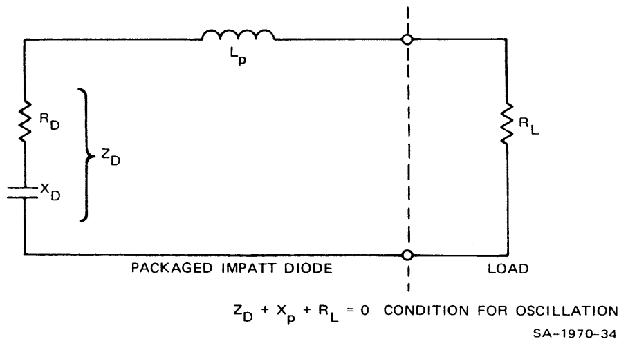
FIGURE V-2 SIMPLE IMPATT DIODE OSCILLATOR CIRCUIT
