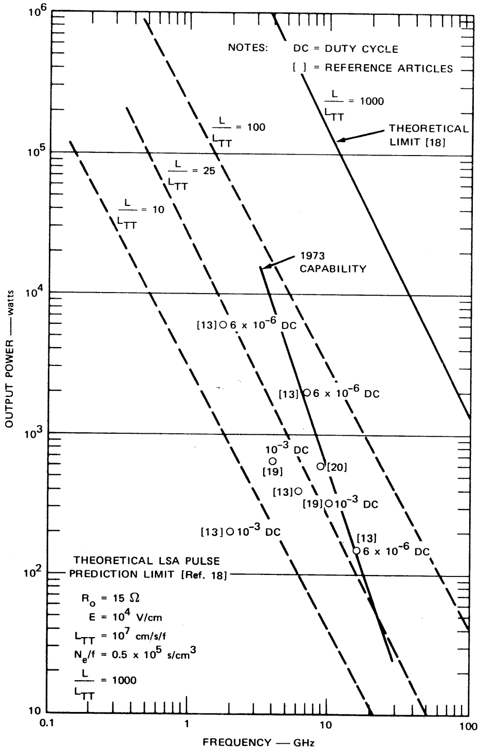
FIGURE VI-4 PERFORMANCE OF LSA DIODES — 1973
