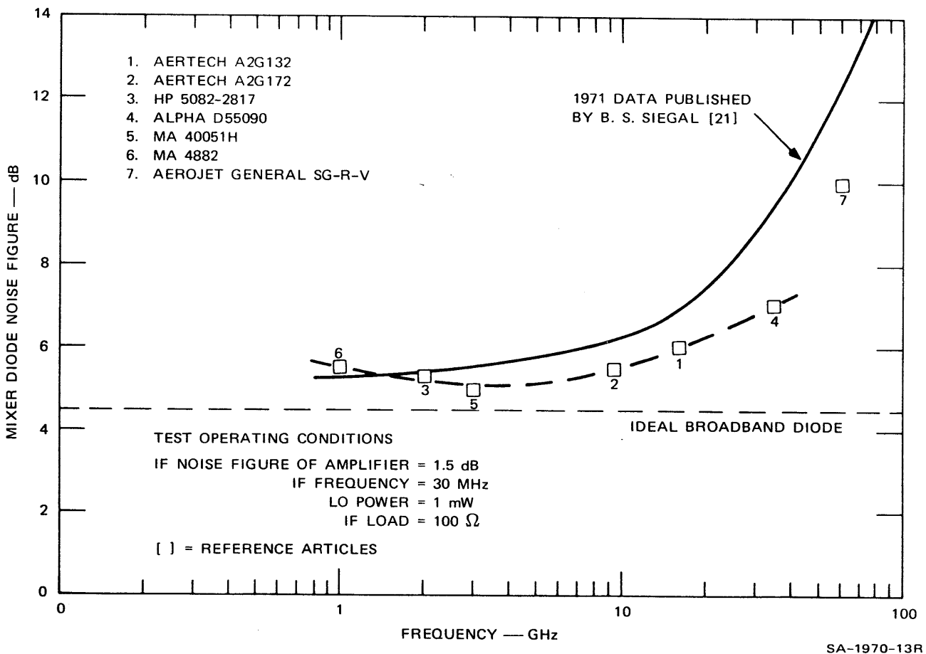
FIGURE VI-5 NOISE-FIGURE PERFORMANCE OF COMMERCIAL SCHOTTKY BARRIER MIXER DIODES — 1973
