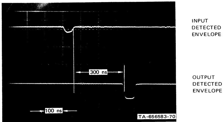
FIGURE V-20 DELAY BETWEEN INPUT AND OUTPUT PULSED RF SIGNALS TO THE BEACON TRANSPONDER
