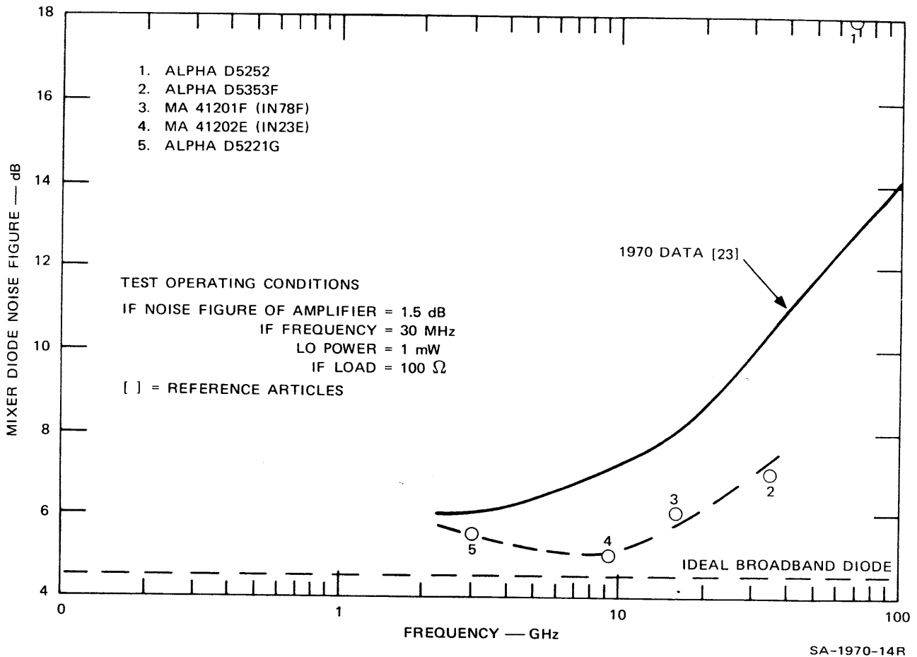
FIGURE VI-6 NOISE-FIGURE PERFORMANCE OF COMMERCIAL POINT CONTACT MIXER DIODES — 1973
