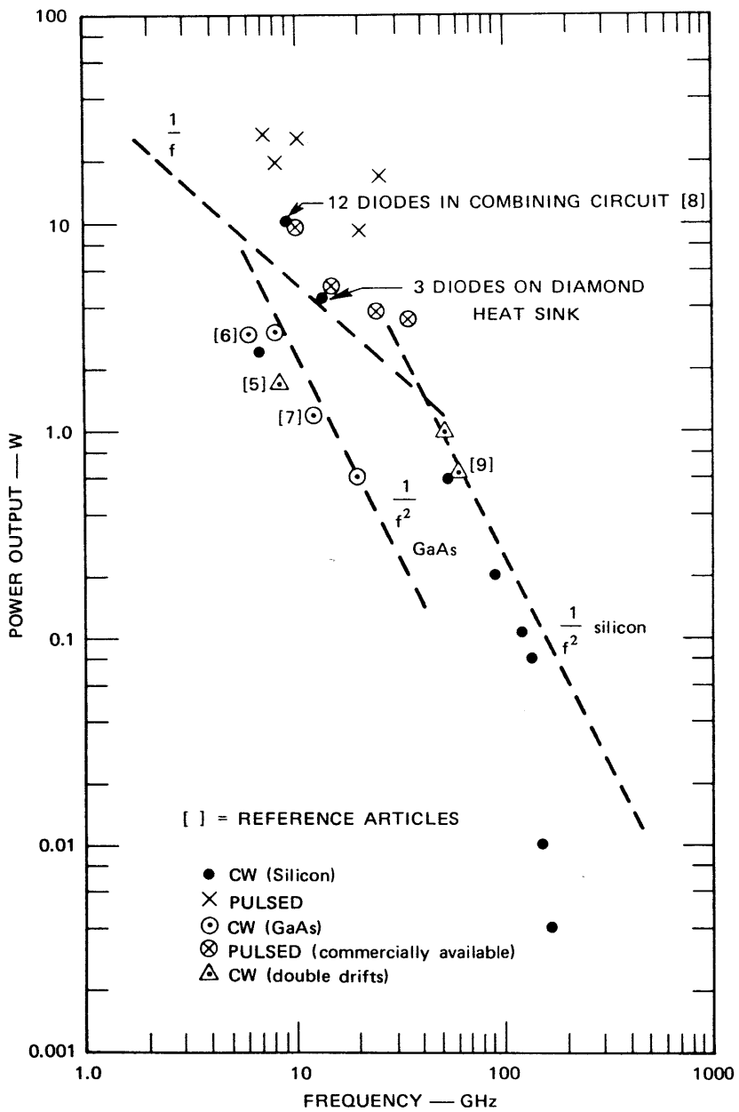
FIGURE VI-1 PERFORMANCE OF IMPATT DIODES — 1973
