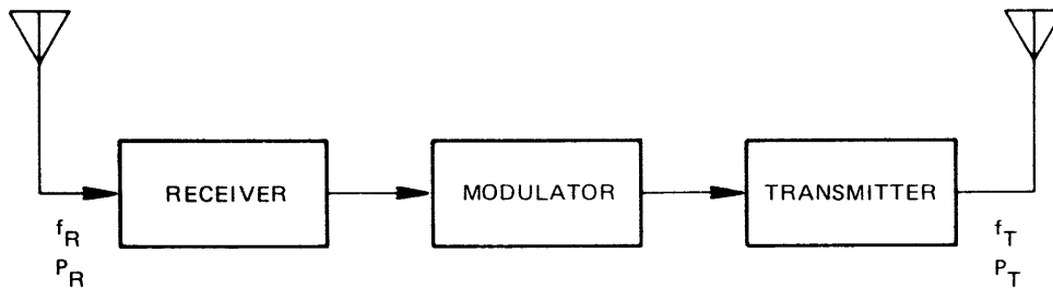
(a) TWO-ANTENNA TRANSPONDER
