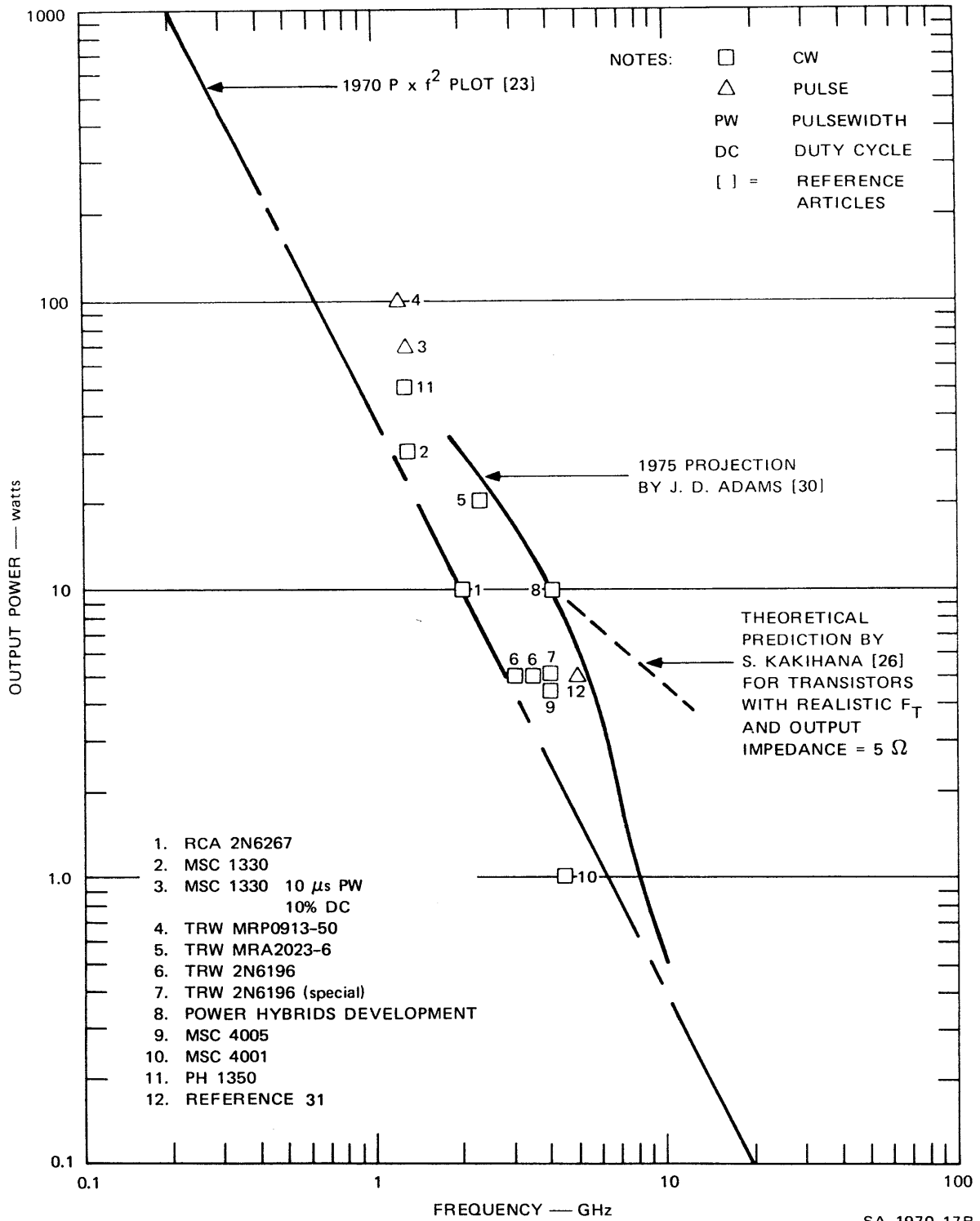
FIGURE VI-9 POWER AS A FUNCTION OF FREQUENCY OF COMMERCIAL MICROWAVE TRANSISTORS — 1973
