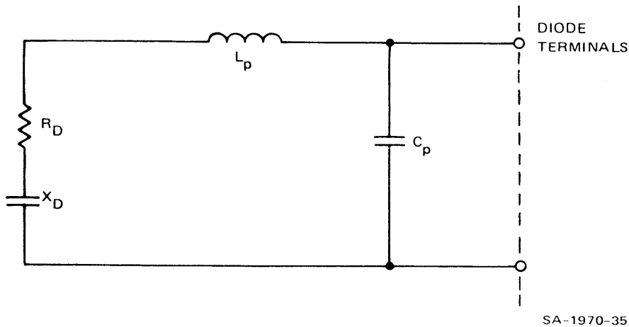
FIGURE V-3 IMPATT DIODE PACKAGE EQUIVALENT CIRCUIT
