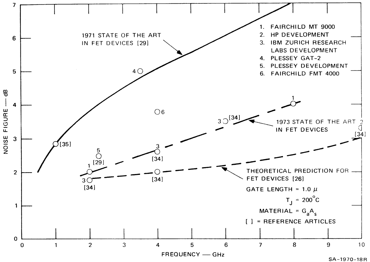
FIGURE VI-10 NOISE-FIGURE PERFORMANCE OF FET DEVICES — 1973
