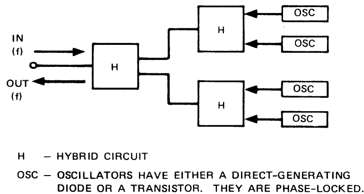
FIGURE VII-5 POWER-COMBINER SCHEME FOR OSCILLATORS USING HYBRIDS
