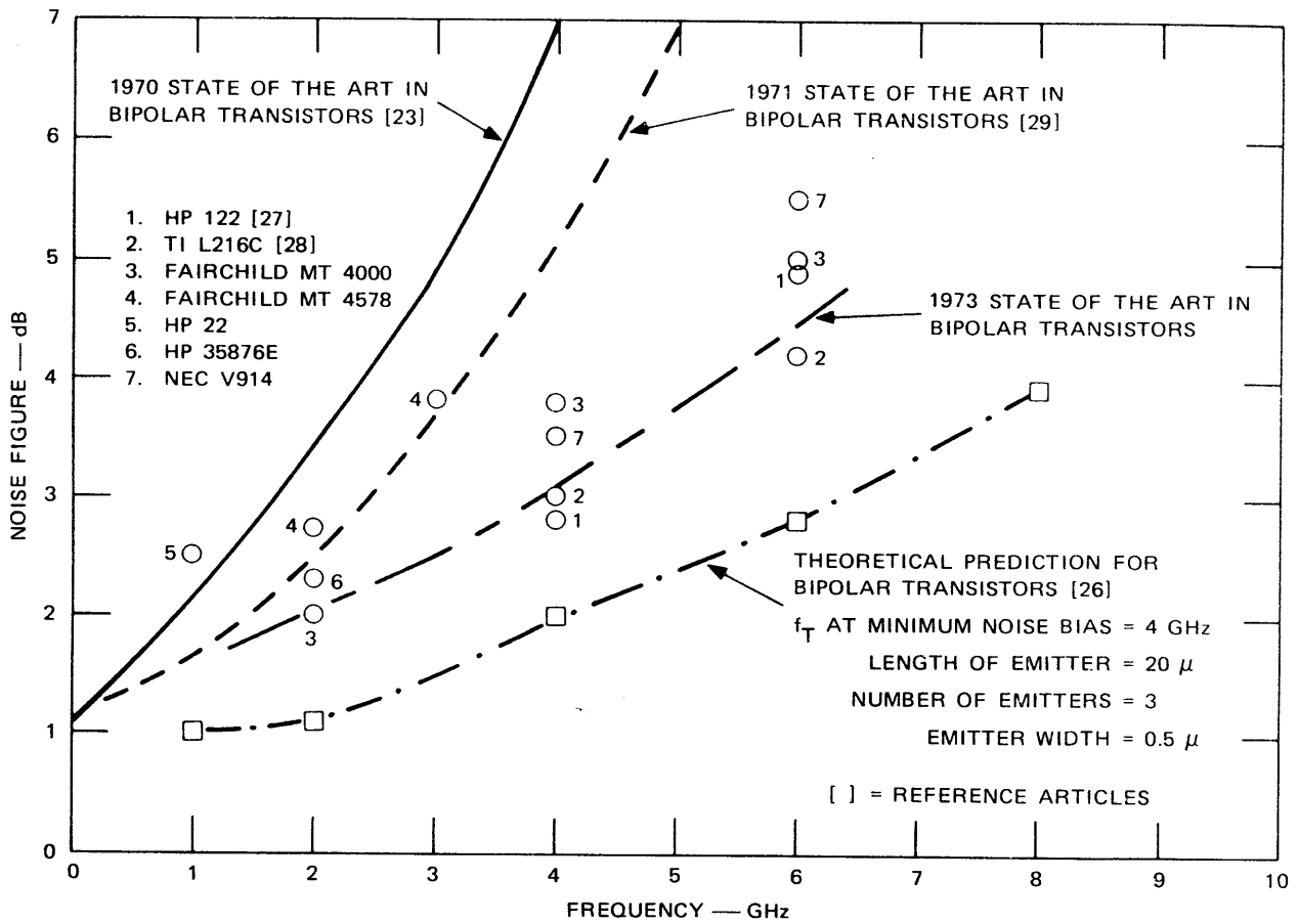
FIGURE VI-8 NOISE-FIGURE PERFORMANCE OF COMMERCIAL BIPOLAR TRANSISTORS — 1973
