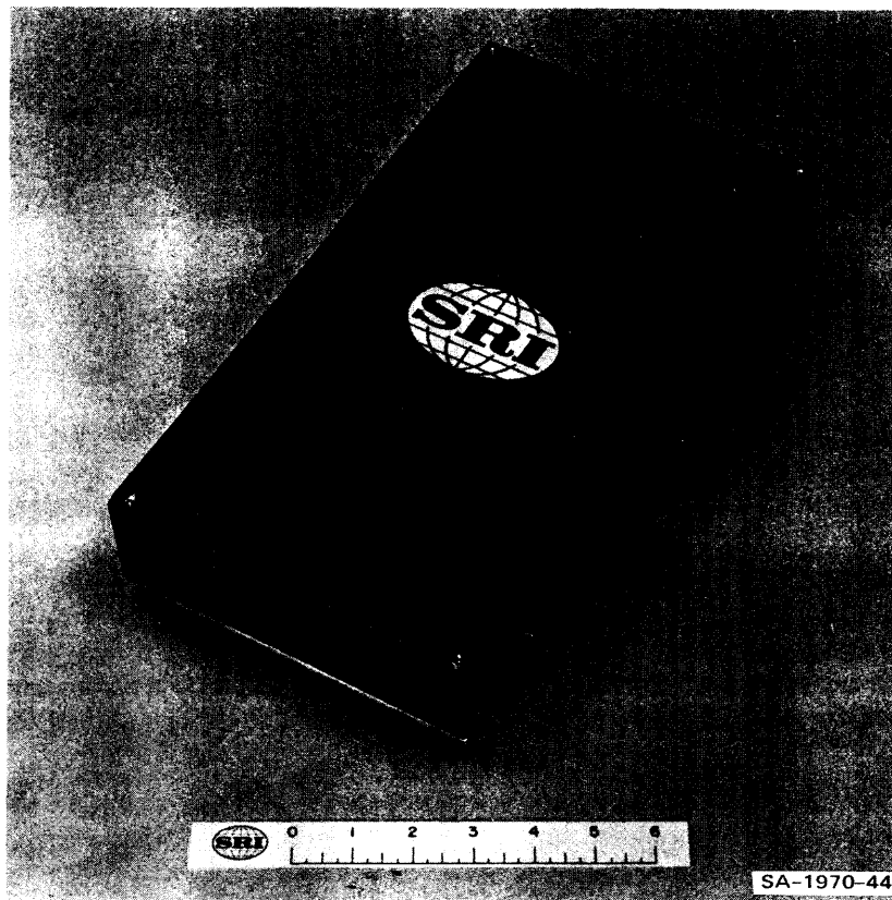
FIGURE V-14 BREADBOARD BEACON TRANSPONDER IN A BOX
