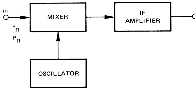
(b) SUPERHETERODYNE RECEIVER
