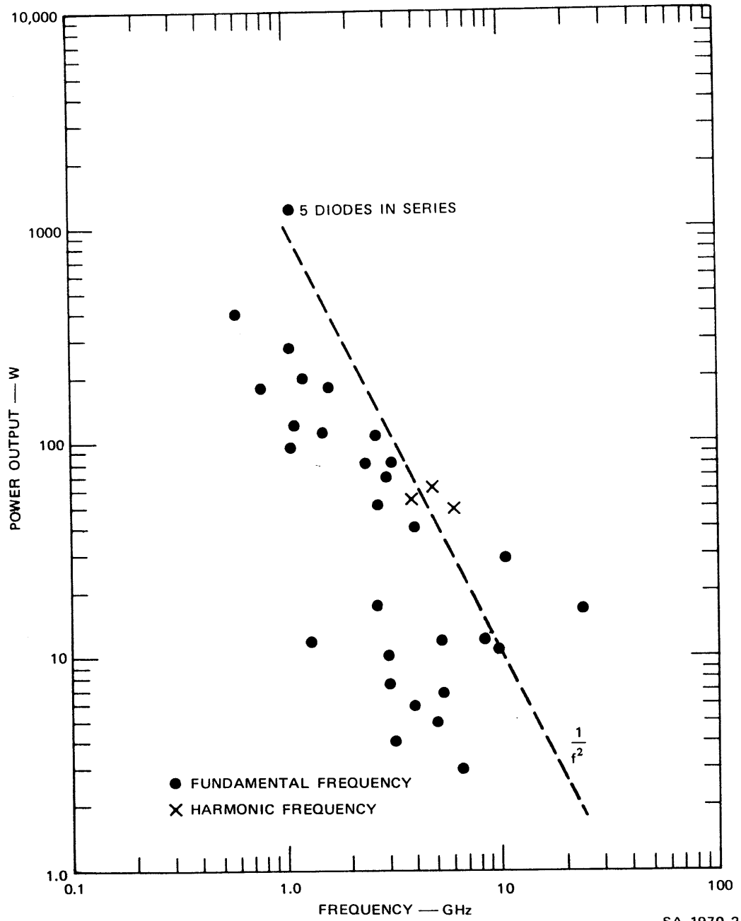
FIGURE VI-2 PERFORMANCE OF TRAPATT DIODES — 1973
