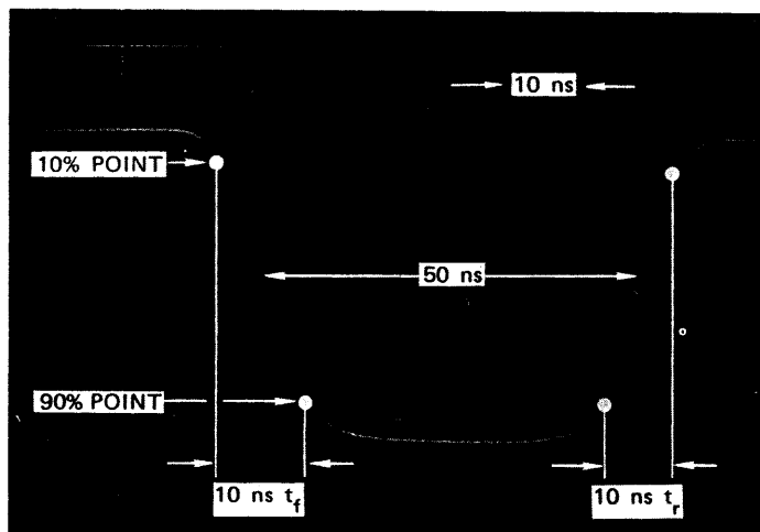
FIGURE V-19 DETECTED ENVELOPE OF RF OUTPUT FROM THE BEACON TRANSPONDER
