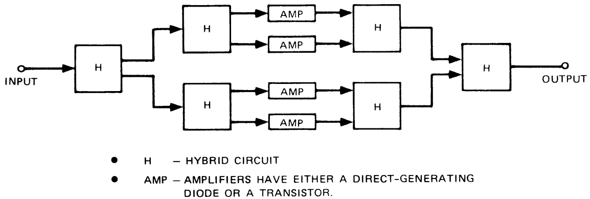
FIGURE VII-4 POWER-COMBINER SCHEME FOR AMPLIFIERS USING HYBRIDS
