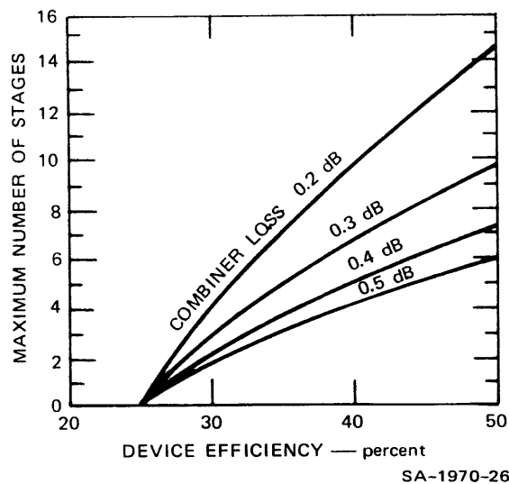
FIGURE VII-7 MAXIMUM NUMBER OF COMBINER STAGES FOR A REQUIRED SYSTEM EFFICIENCY OF 25 PERCENT. Source: Ref. 1.
