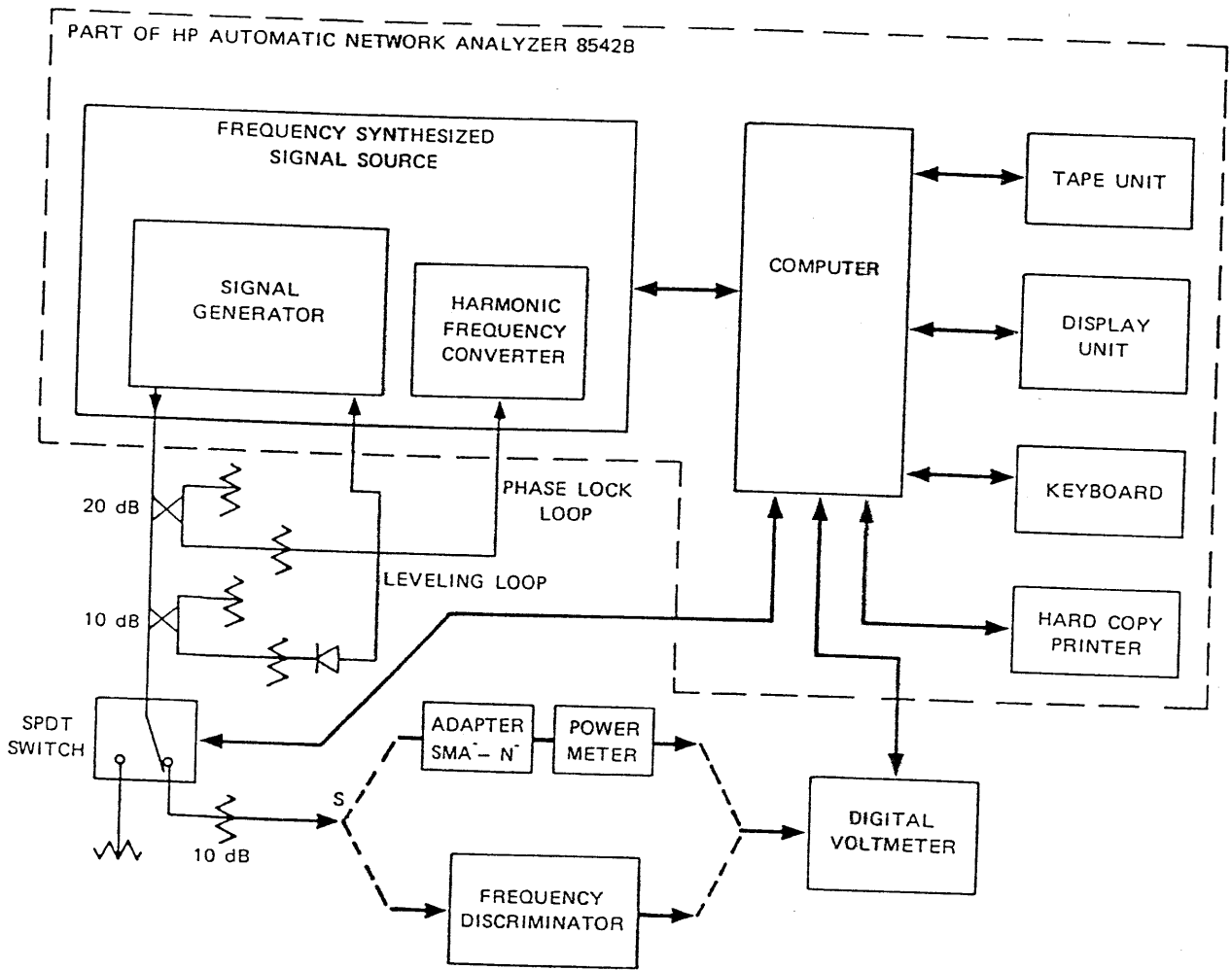
FIGURE 32 BLOCK DIAGRAM OF DISCRIMINATOR MEASUREMENT TEST SETUP
