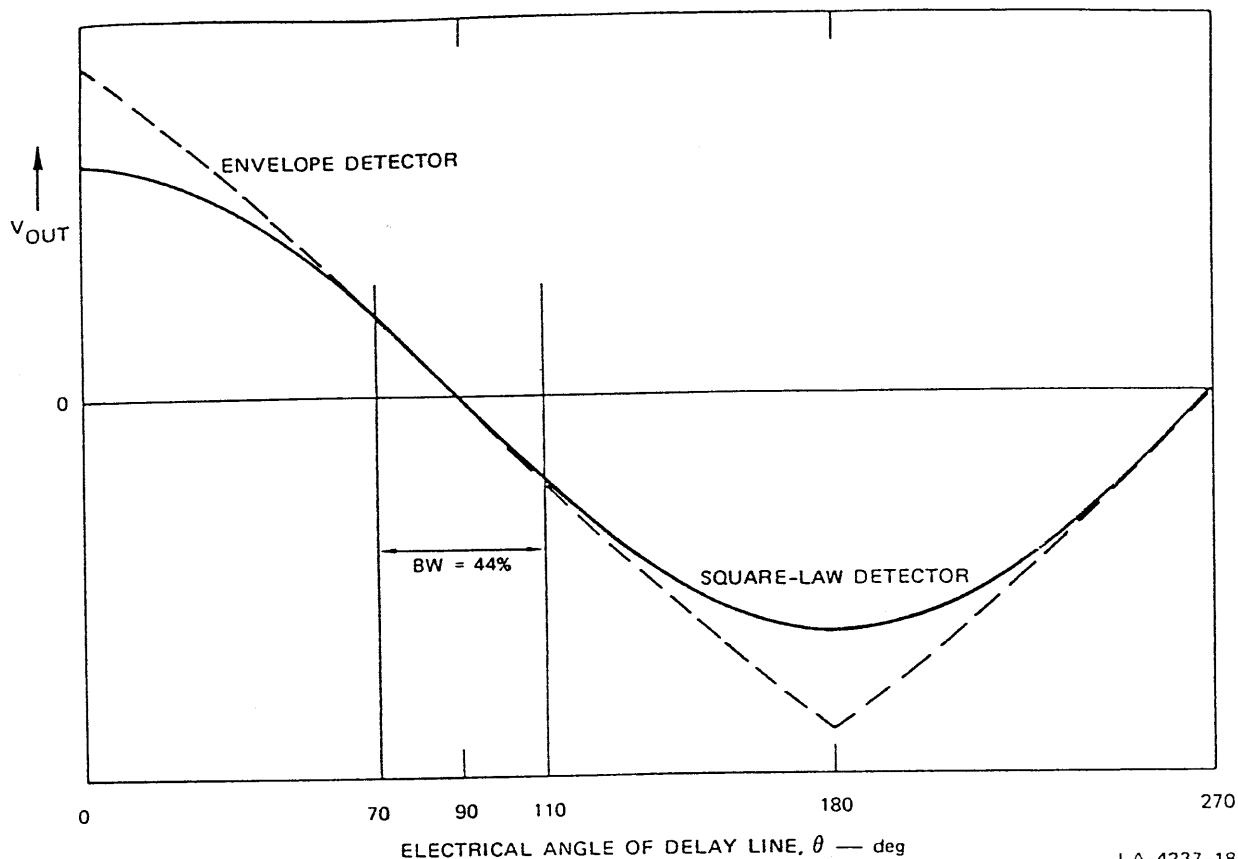
FIGURE 2 COMPARISON BETWEEN DISCRIMINATORS USING SQUARE-LAW AND ENVELOPE DETECTORS ( k = 1 )
