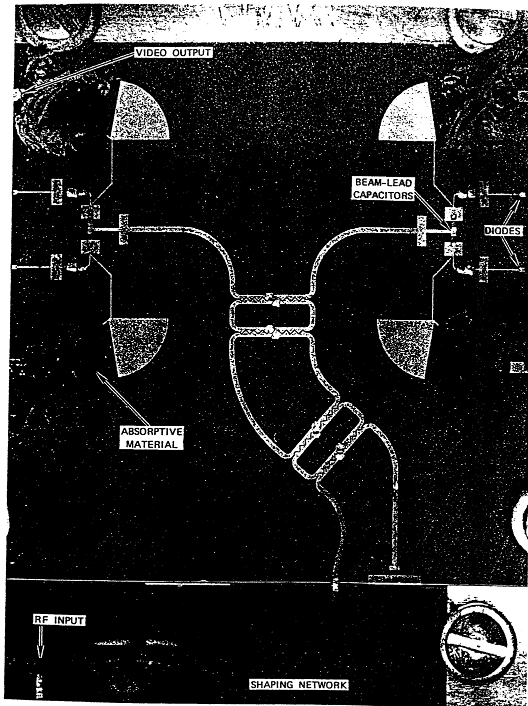
FIGURE 11 PHOTOGRAPH OF THE FREQUENCY-DISCRIMINATOR MIC CIRCUIT WITH SHAPING NETWORK (Model 2)
