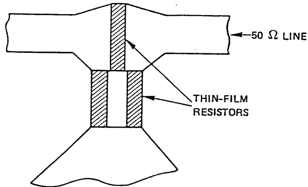
(c) MODIFIED GEOMETRY WITH WIDER SERIES-RESISTOR GAP
