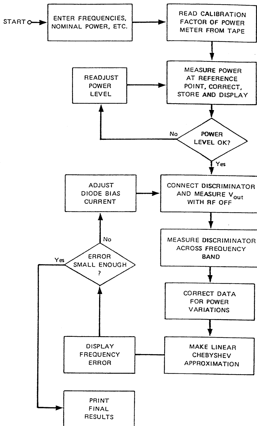
FIGURE 33 FLOW DIAGRAM OF DISCRIMINATOR MEASUREMENT PROGRAM
