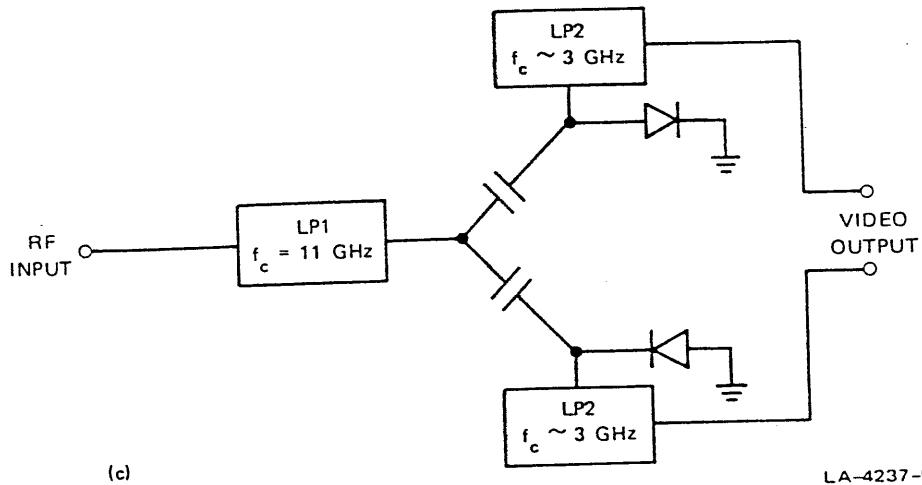
FIGURE 17 THREE DETECTOR CIRCUITS WITH REACTIVELY TERMINATED HARMONICS
