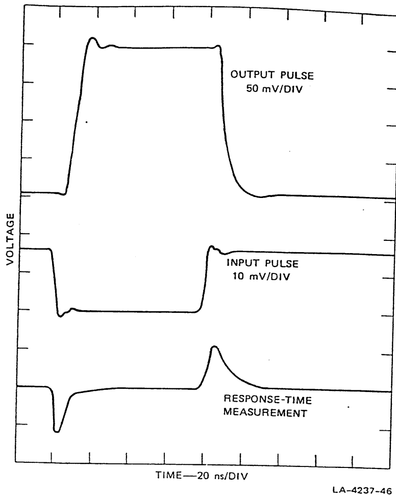
FIGURE 31 PULSE RESPONSE OF DIFFERENTIAL VIDEO AMPLIFIER
