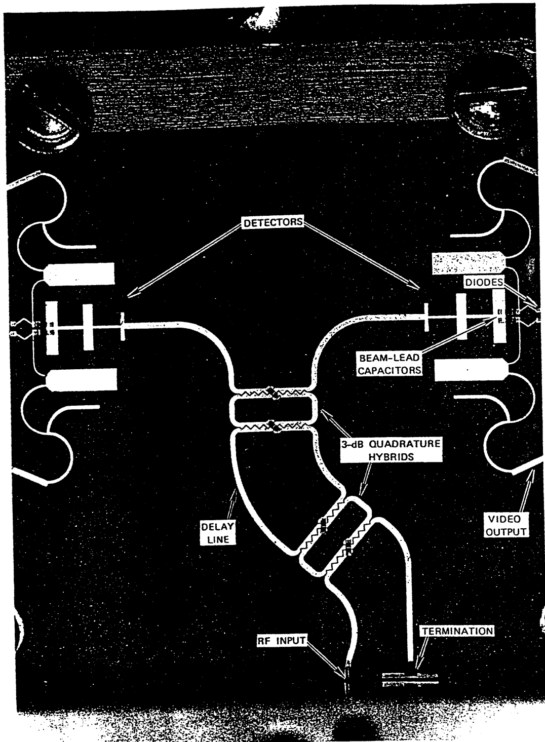
FIGURE 6 PHOTOGRAPH OF THE FREQUENCY-DISCRIMINATOR MIC CIRCUIT (Model 1)
