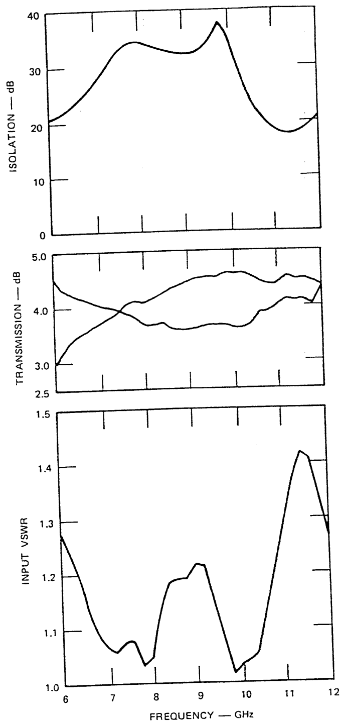
FIGURE 15 MEASURED CHARACTERISTICS OF 3-dB QUADRATURE HYBRID
