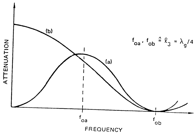
FIGURE 25 TWO SHAPING-NETWORK TOPOLOGIES
