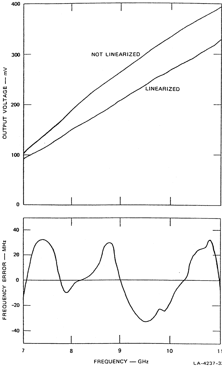
FIGURE 13 OUTPUT VOLTAGE AND FREQUENCY ERROR OF LINEARIZED DISCRIMINATOR, MODEL 2
