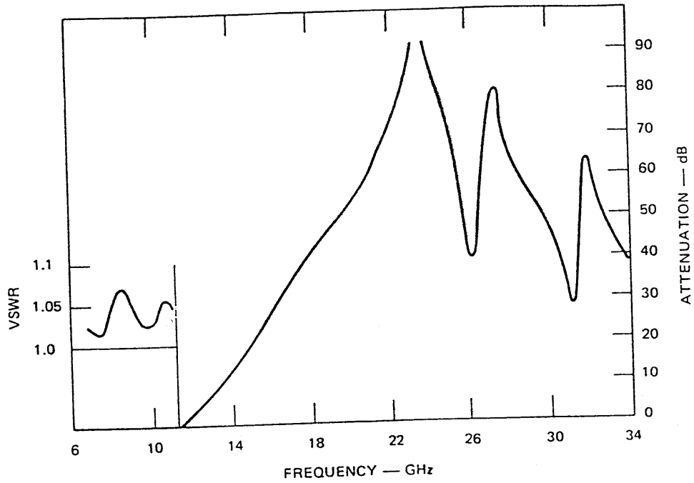
(a) VSWR AND ATTENUATION
