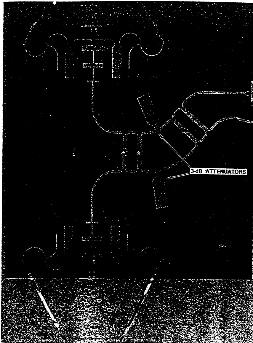
FIGURE 8 PHOTOGRAPH OF THE FREQUENCY-DISCRIMINATOR MIC CIRCUIT (Model 1a)
