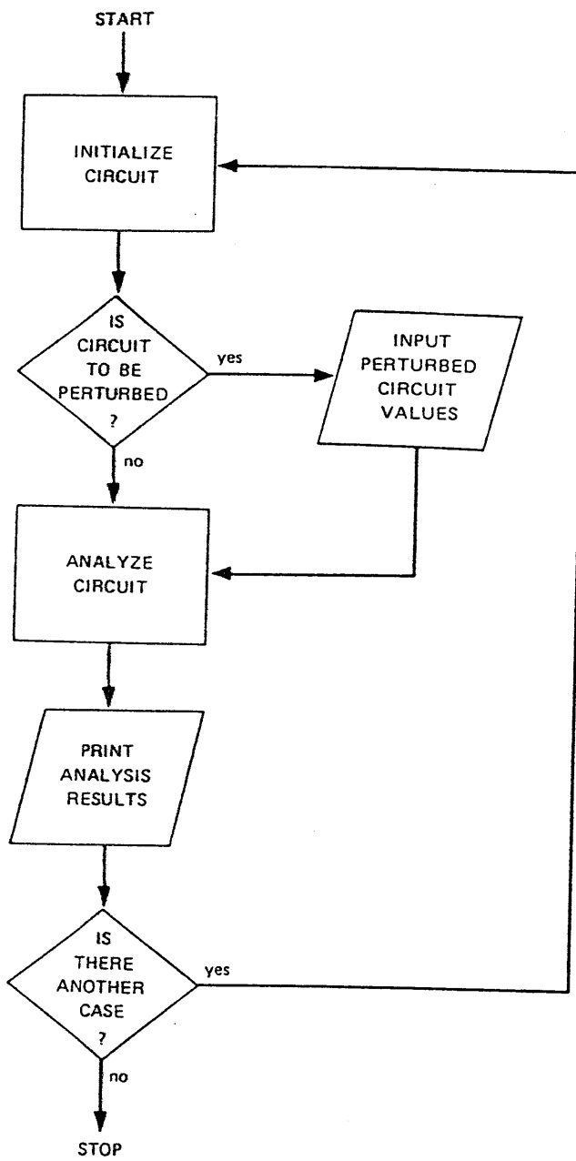
FIGURE 4 FLOWCHART FOR FREQUENCY-DISCRIMINATOR ANALYSIS PROGRAM
