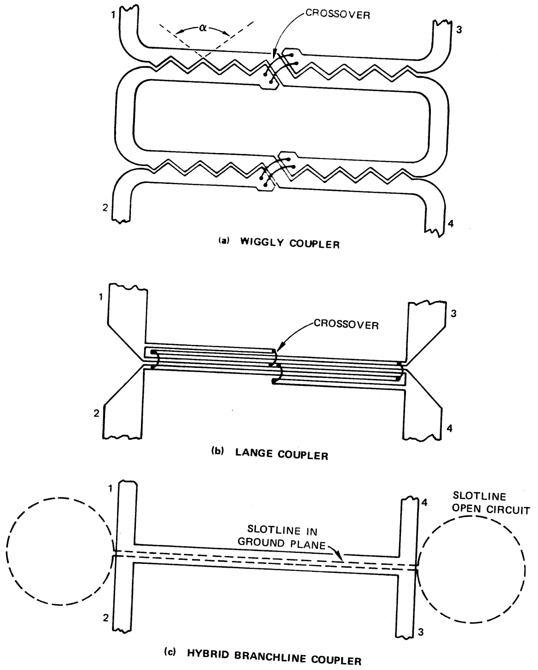
FIGURE 14 THREE POSSIBLE MIC QUADRATURE HYBRIDS
