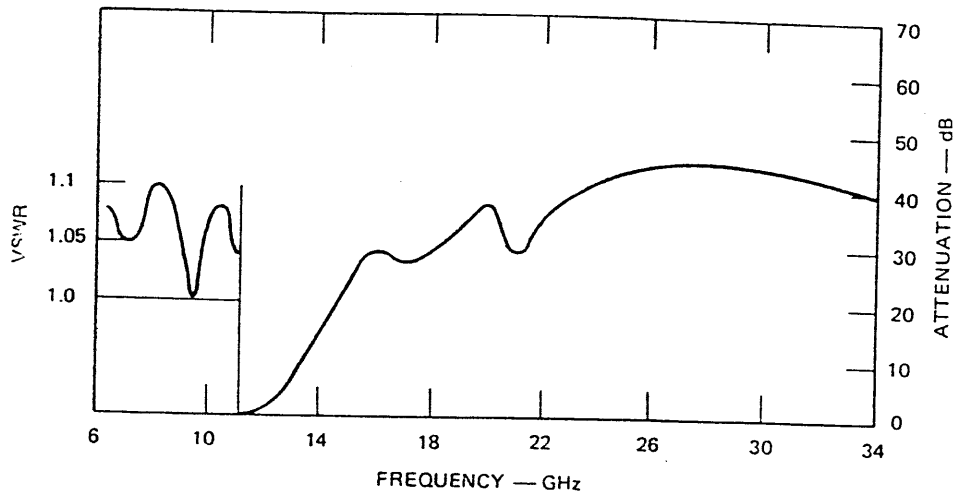
(a) VSWR AND ATTENUATION
