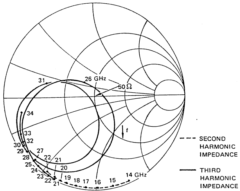
(b) HARMONIC IMPEDANCES SEEN BY R_i
