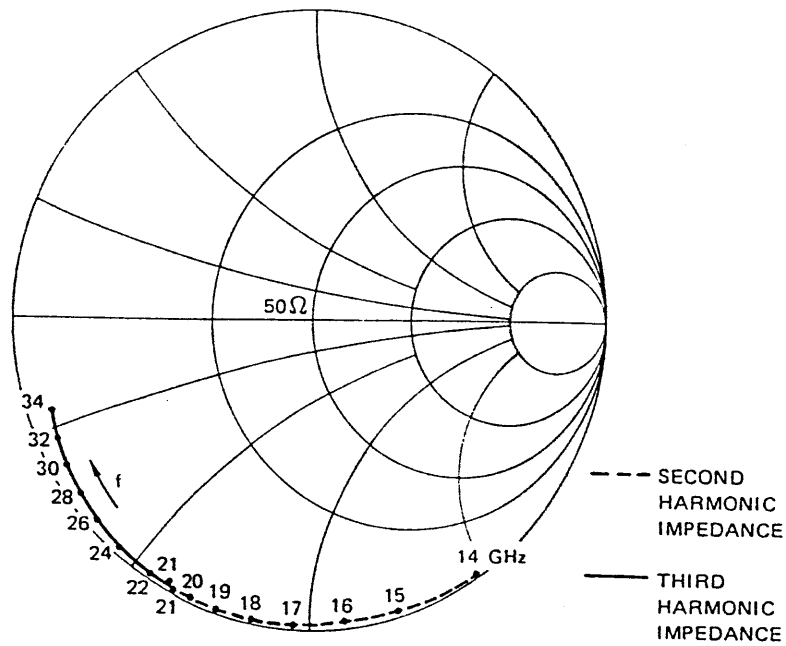
(b) HARMONIC IMPEDANCES SEEN BY R_i
