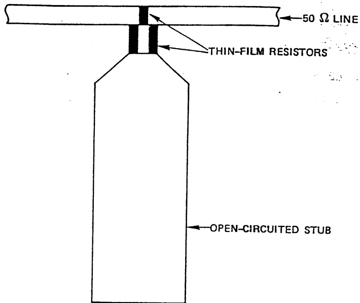
(b) MICROWAVE IMPLEMENTATION OF ATTENUATOR
