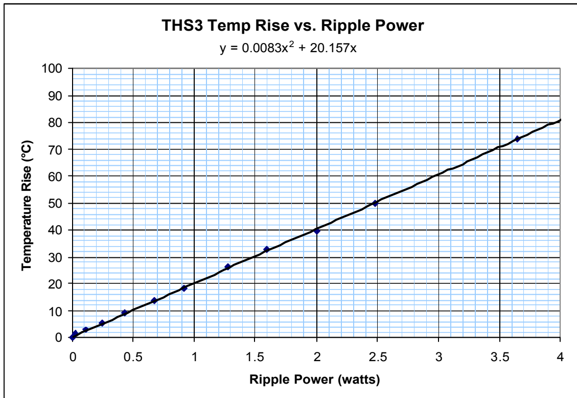
Figure 8. Temperature rise vs. ripple power dissipation for THQ3.
