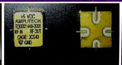
0.1-6.0 GHz Surface Mount LNA (>25 dB Gain)
